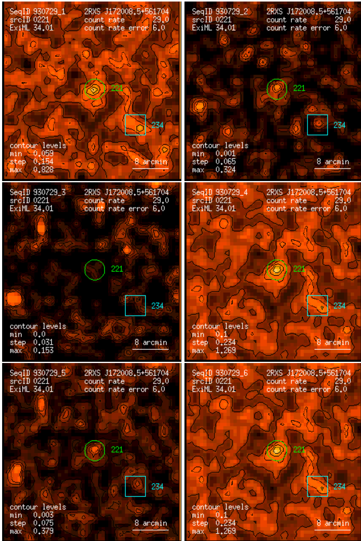
Figure 221: RASS 930729: detection 0221: band rate images, Gaussian filter: (1) PSPC channels 11 – 41, (2) 52 – 90, (3) 91 – 201, (4) 11 – 235, (5) 52 – 201, (6) 11 – 201. Broad band rates in counts/ks. Band rate contour levels in counts/ks/arcmin 2 .
