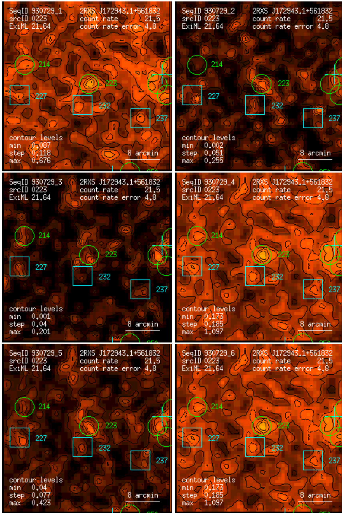
Figure 223: RASS 930729: detection 0223: band rate images, Gaussian filter: (1) PSPC channels 11 – 41, (2) 52 – 90, (3) 91 – 201, (4) 11 – 235, (5) 52 – 201, (6) 11 – 201. Broad band rates in counts/ks. Band rate contour levels in counts/ks/arcmin 2 .
