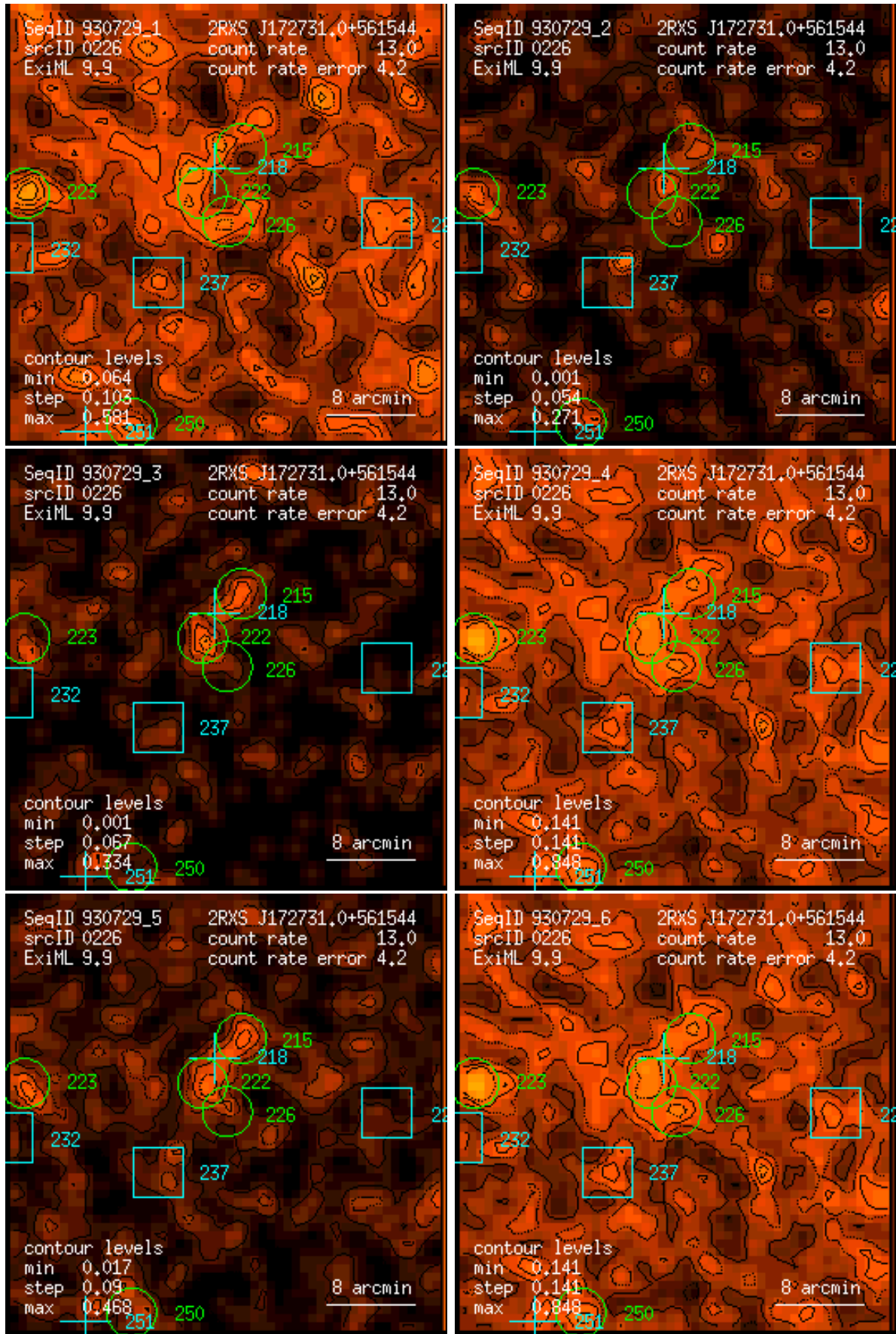
Figure 226: RASS 930729: detection 0226: band rate images, Gaussian filter: (1) PSPC channels 11 – 41, (2) 52 – 90, (3) 91 – 201, (4) 11 – 235, (5) 52 – 201, (6) 11 – 201. Broad band rates in counts/ks. Band rate contour levels in counts/ks/arcmin 2 .
