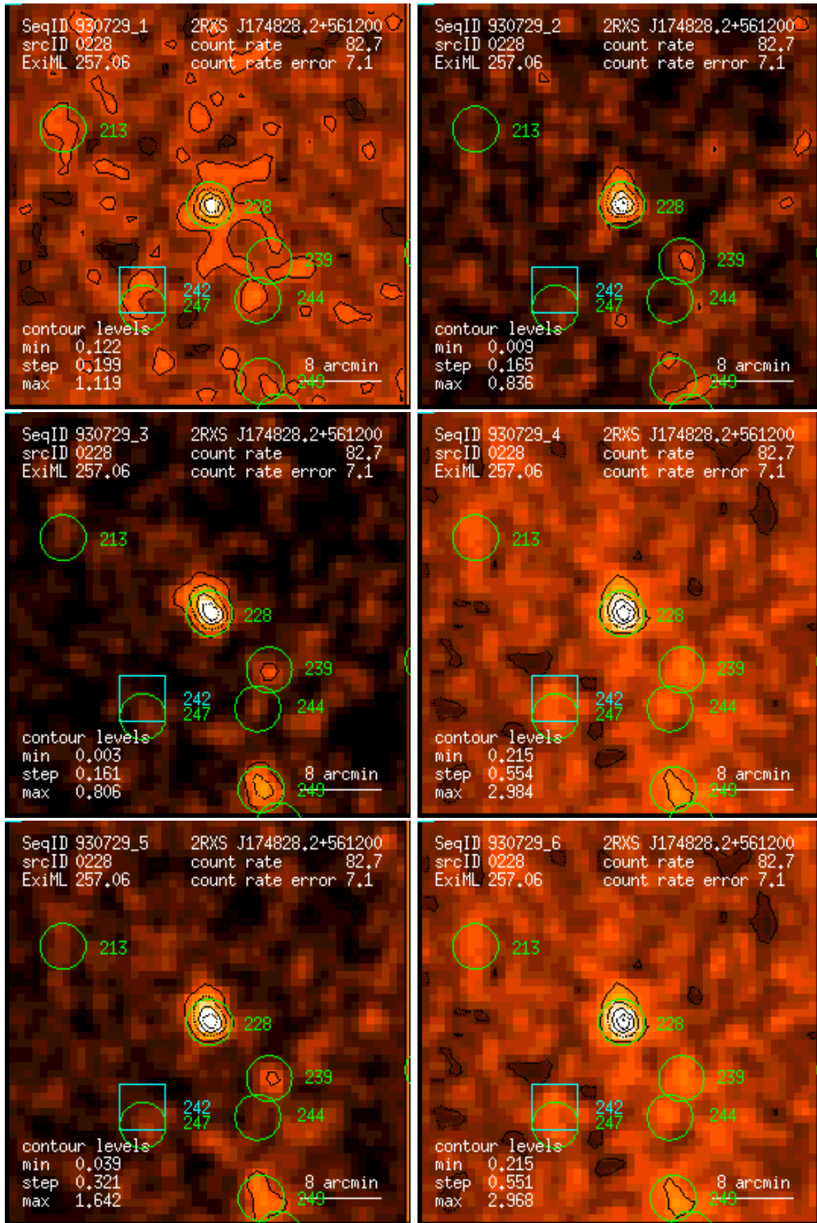
Figure 228: RASS 930729: detection 0228: band rate images, Gaussian filter: (1) PSPC channels 11 – 41, (2) 52 – 90, (3) 91 – 201, (4) 11 – 235, (5) 52 – 201, (6) 11 – 201. Broad band rates in counts/ks. Band rate contour levels in counts/ks/arcmin 2 .
