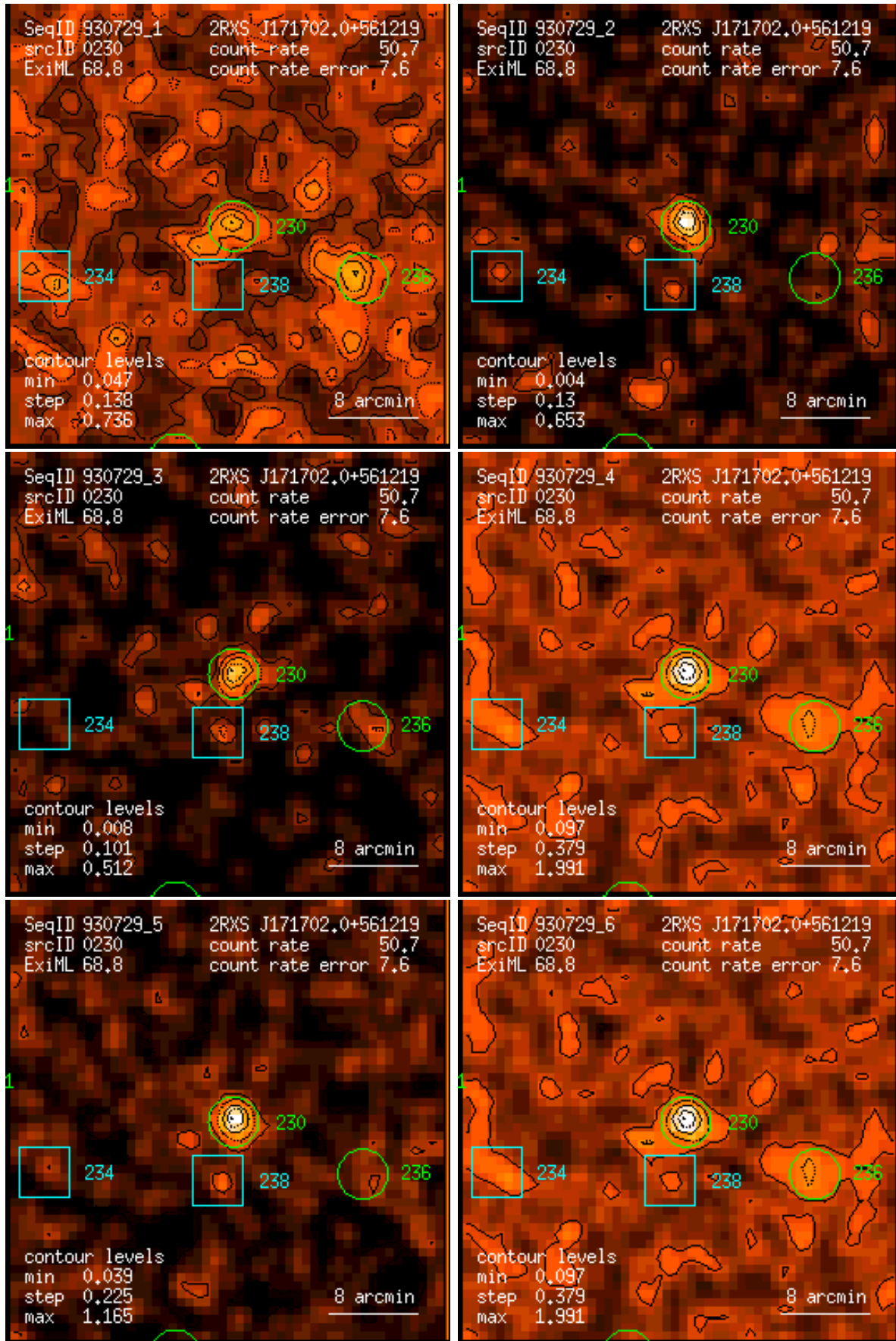
Figure 230: RASS 930729: detection 0230: band rate images, Gaussian filter: (1) PSPC channels 11 – 41, (2) 52 – 90, (3) 91 – 201, (4) 11 – 235, (5) 52 – 201, (6) 11 – 201. Broad band rates in counts/ks. Band rate contour levels in counts/ks/arcmin 2 .
