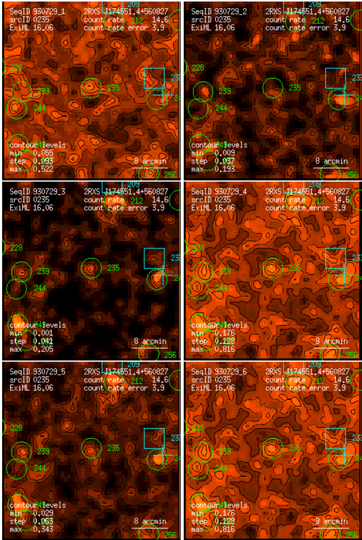
Figure 235: RASS 930729: detection 0235: band rate images, Gaussian filter: (1) PSPC channels 11 – 41, (2) 52 – 90, (3) 91 – 201, (4) 11 – 235, (5) 52 – 201, (6) 11 – 201. Broad band rates in counts/ks. Band rate contour levels in counts/ks/arcmin 2 .
