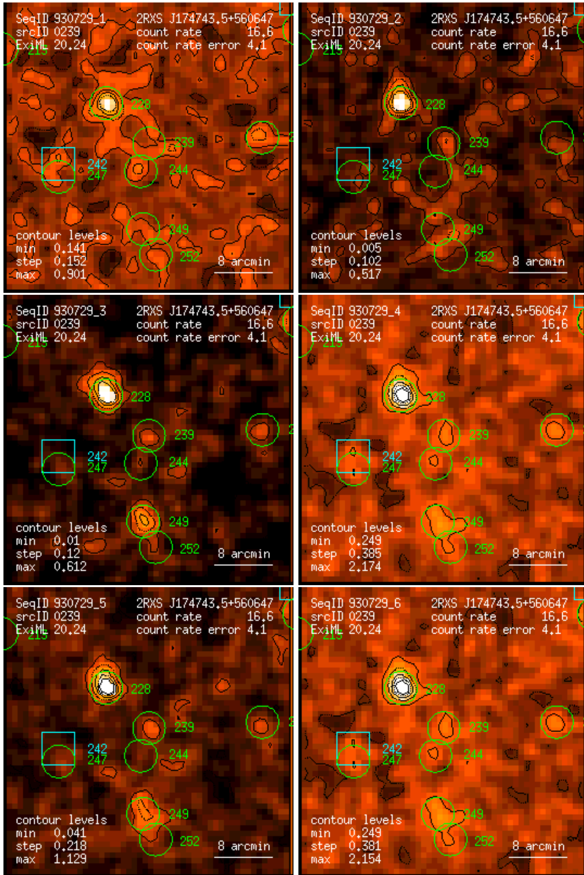
Figure 239: RASS 930729: detection 0239: band rate images, Gaussian filter: (1) PSPC channels 11 – 41, (2) 52 – 90, (3) 91 – 201, (4) 11 – 235, (5) 52 – 201, (6) 11 – 201. Broad band rates in counts/ks. Band rate contour levels in counts/ks/arcmin 2 .
