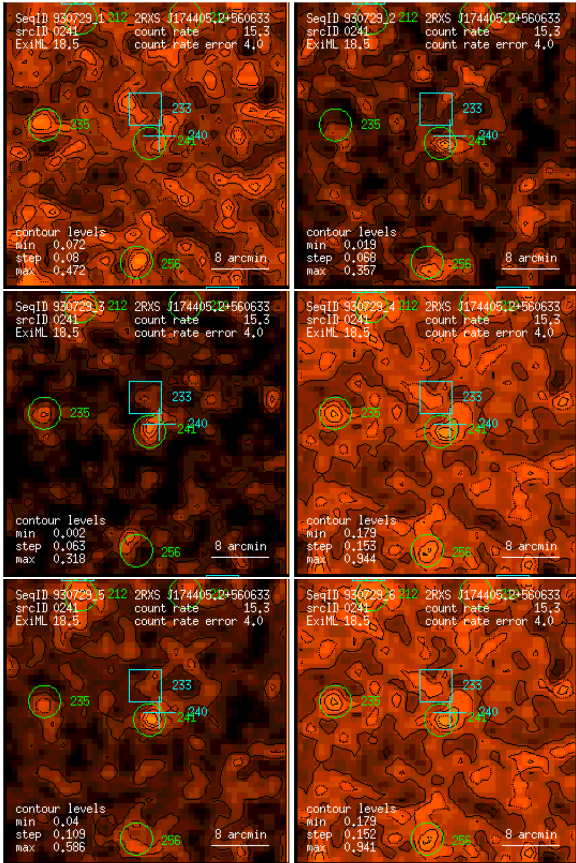
Figure 241: RASS 930729: detection 0241: band rate images, Gaussian filter: (1) PSPC channels 11 – 41, (2) 52 – 90, (3) 91 – 201, (4) 11 – 235, (5) 52 – 201, (6) 11 – 201. Broad band rates in counts/ks. Band rate contour levels in counts/ks/arcmin 2 .
