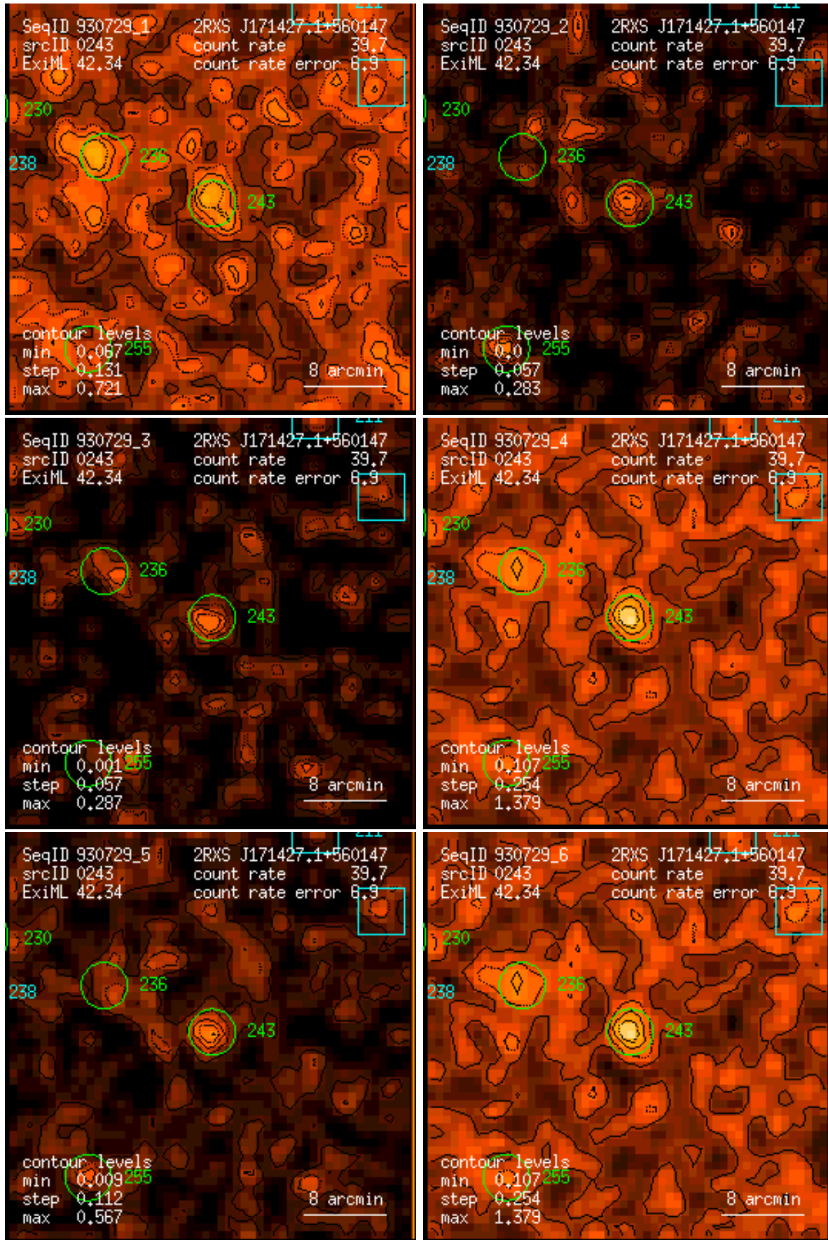
Figure 243: RASS 930729: detection 0243: band rate images, Gaussian filter: (1) PSPC channels 11 – 41, (2) 52 – 90, (3) 91 – 201, (4) 11 – 235, (5) 52 – 201, (6) 11 – 201. Broad band rates in counts/ks. Band rate contour levels in counts/ks/arcmin 2 .
