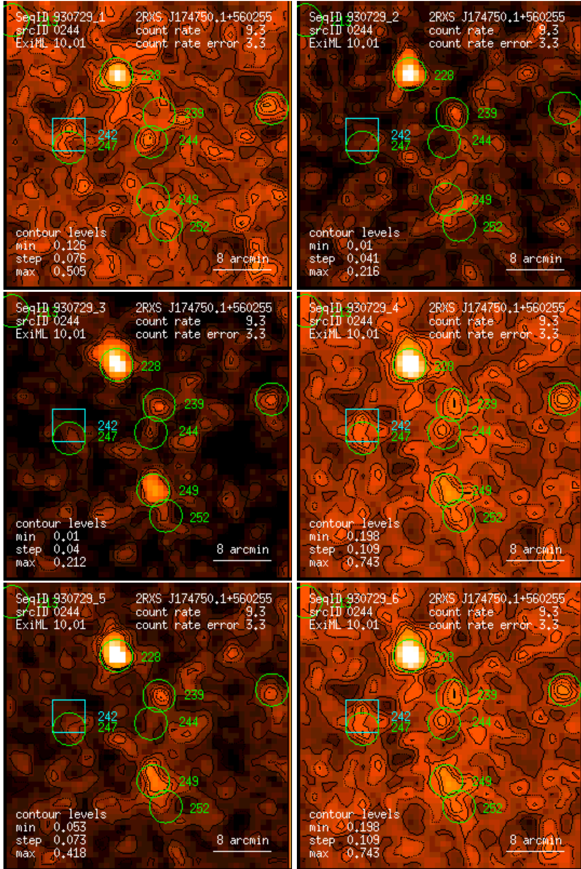
Figure 244: RASS 930729: detection 0244: band rate images, Gaussian filter: (1) PSPC channels 11 – 41, (2) 52 – 90, (3) 91 – 201, (4) 11 – 235, (5) 52 – 201, (6) 11 – 201. Broad band rates in counts/ks. Band rate contour levels in counts/ks/arcmin 2 .
