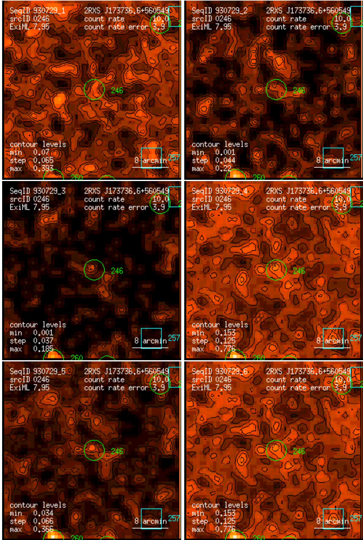
Figure 246: RASS 930729: detection 0246: band rate images, Gaussian filter: (1) PSPC channels 11 – 41, (2) 52 – 90, (3) 91 – 201, (4) 11 – 235, (5) 52 – 201, (6) 11 – 201. Broad band rates in counts/ks. Band rate contour levels in counts/ks/arcmin 2 .
