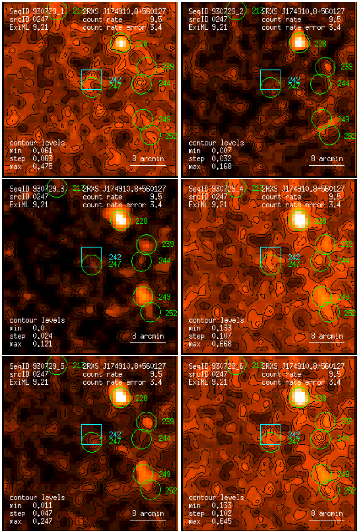
Figure 247: RASS 930729: detection 0247: band rate images, Gaussian filter: (1) PSPC channels 11 – 41, (2) 52 – 90, (3) 91 – 201, (4) 11 – 235, (5) 52 – 201, (6) 11 – 201. Broad band rates in counts/ks. Band rate contour levels in counts/ks/arcmin 2 .
