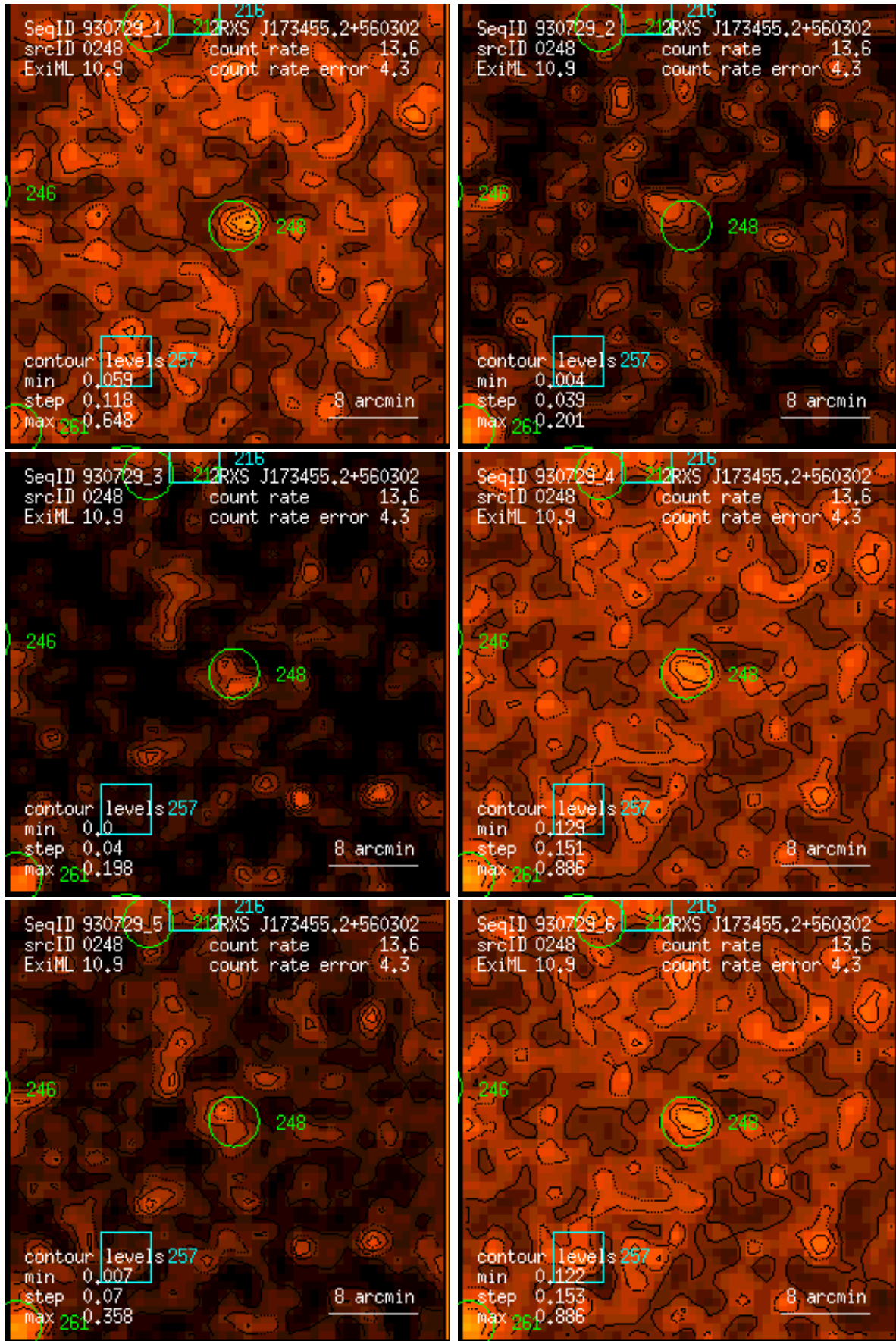
Figure 248: RASS 930729: detection 0248: band rate images, Gaussian filter: (1) PSPC channels 11 – 41, (2) 52 – 90, (3) 91 – 201, (4) 11 – 235, (5) 52 – 201, (6) 11 – 201. Broad band rates in counts/ks. Band rate contour levels in counts/ks/arcmin 2 .
