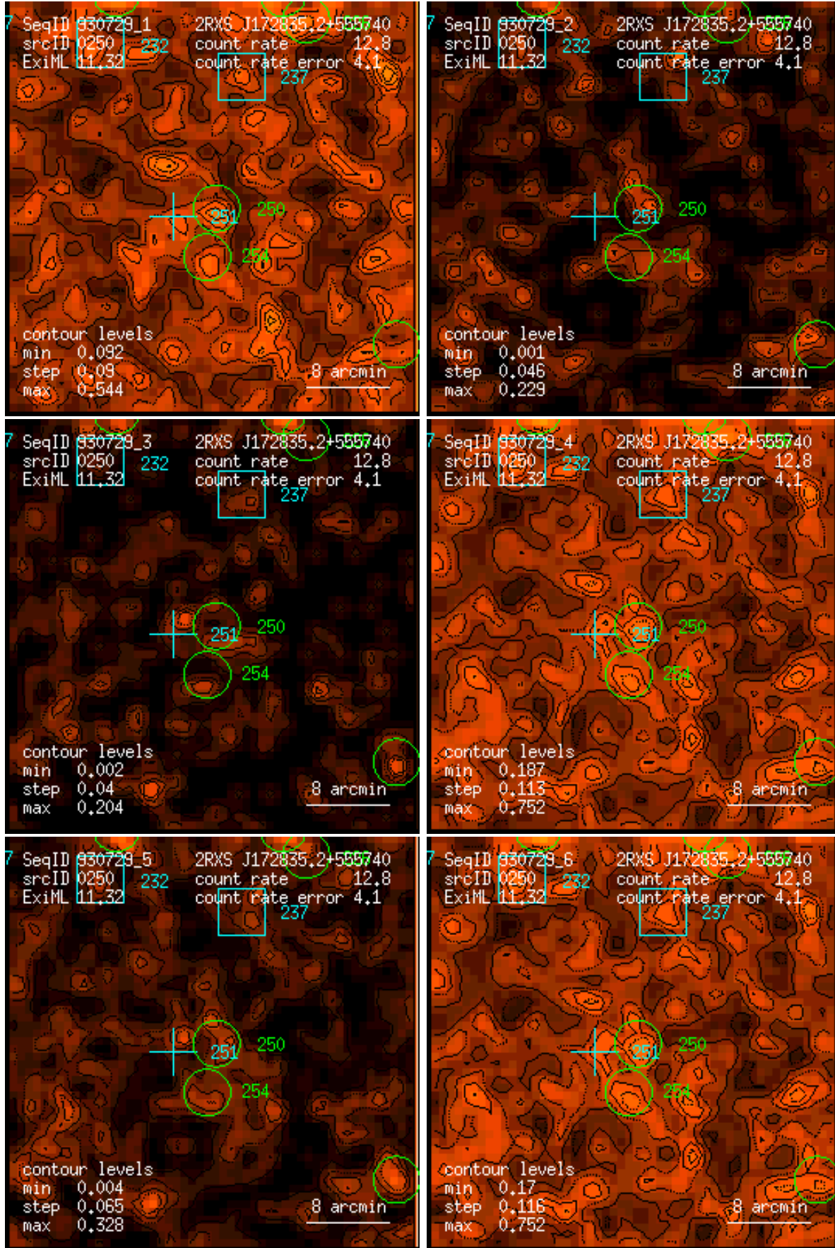
Figure 250: RASS 930729: detection 0250: band rate images, Gaussian filter: (1) PSPC channels 11 – 41, (2) 52 – 90, (3) 91 – 201, (4) 11 – 235, (5) 52 – 201, (6) 11 – 201. Broad band rates in counts/ks. Band rate contour levels in counts/ks/arcmin 2 .
