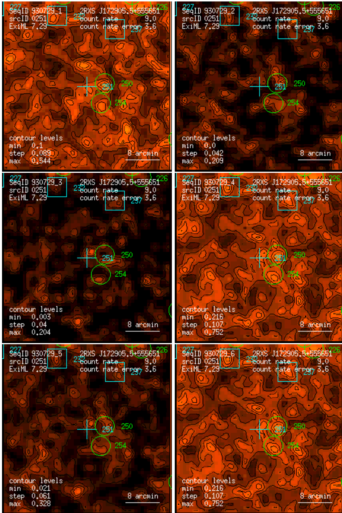
Figure 251: RASS 930729: detection 0251: band rate images, Gaussian filter: (1) PSPC channels 11 – 41, (2) 52 – 90, (3) 91 – 201, (4) 11 – 235, (5) 52 – 201, (6) 11 – 201. Broad band rates in counts/ks. Band rate contour levels in counts/ks/arcmin 2 .
