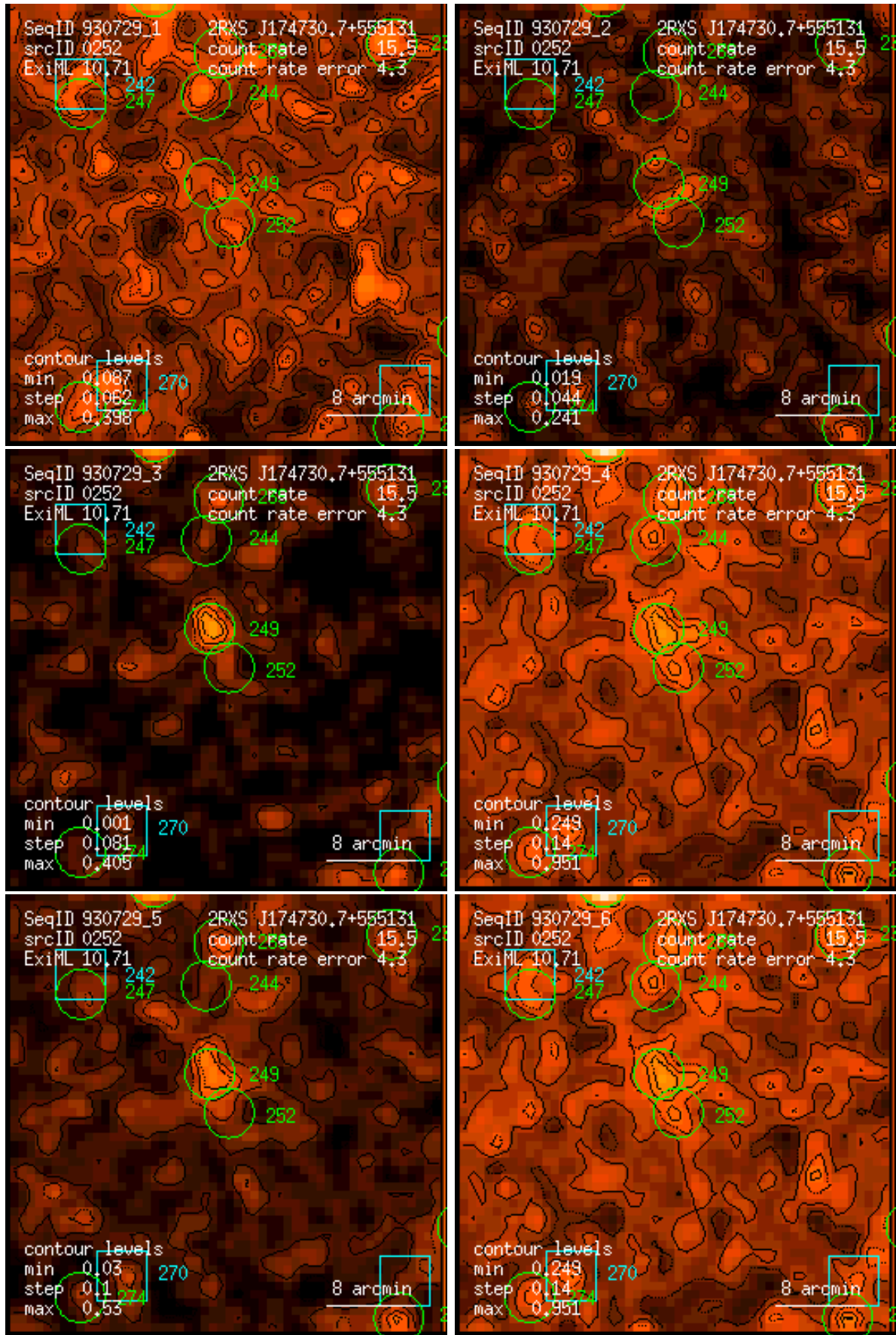
Figure 252: RASS 930729: detection 0252: band rate images, Gaussian filter: (1) PSPC channels 11 – 41, (2) 52 – 90, (3) 91 – 201, (4) 11 – 235, (5) 52 – 201, (6) 11 – 201. Broad band rates in counts/ks. Band rate contour levels in counts/ks/arcmin 2 .
