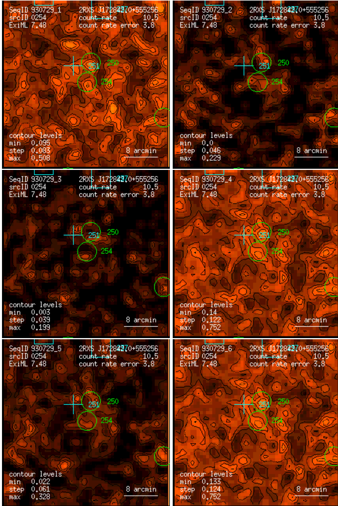
Figure 254: RASS 930729: detection 0254: band rate images, Gaussian filter: (1) PSPC channels 11 – 41, (2) 52 – 90, (3) 91 – 201, (4) 11 – 235, (5) 52 – 201, (6) 11 – 201. Broad band rates in counts/ks. Band rate contour levels in counts/ks/arcmin 2 .
