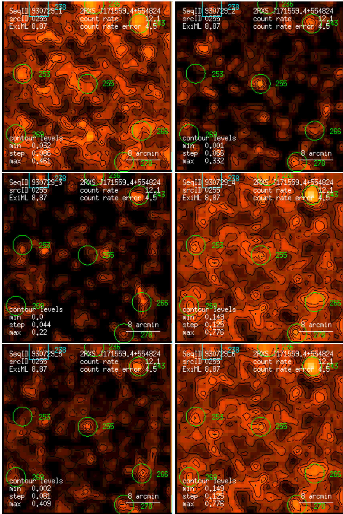
Figure 255: RASS 930729: detection 0255: band rate images, Gaussian filter: (1) PSPC channels 11 – 41, (2) 52 – 90, (3) 91 – 201, (4) 11 – 235, (5) 52 – 201, (6) 11 – 201. Broad band rates in counts/ks. Band rate contour levels in counts/ks/arcmin 2 .
