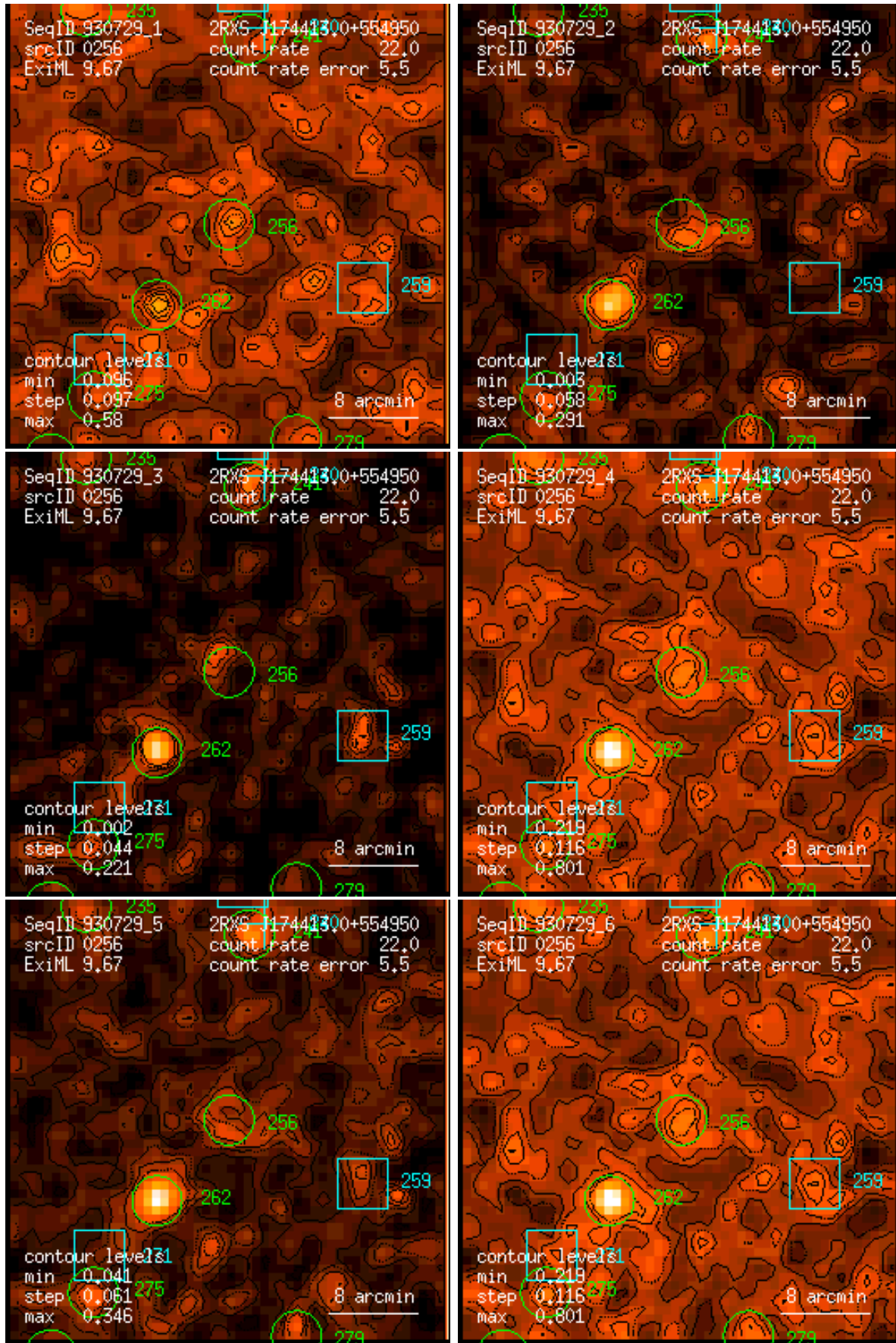
Figure 256: RASS 930729: detection 0256: band rate images, Gaussian filter: (1) PSPC channels 11 – 41, (2) 52 – 90, (3) 91 – 201, (4) 11 – 235, (5) 52 – 201, (6) 11 – 201. Broad band rates in counts/ks. Band rate contour levels in counts/ks/arcmin 2 .
