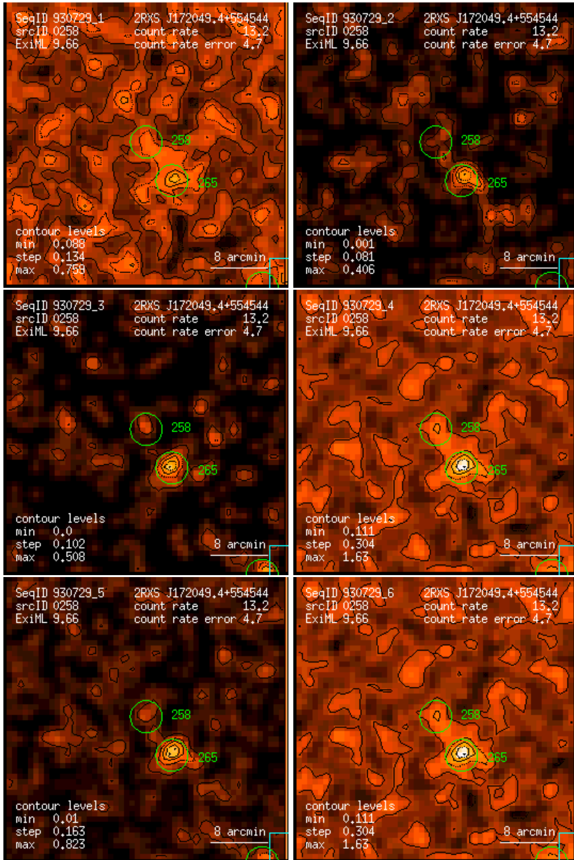
Figure 258: RASS 930729: detection 0258: band rate images, Gaussian filter: (1) PSPC channels 11 – 41, (2) 52 – 90, (3) 91 – 201, (4) 11 – 235, (5) 52 – 201, (6) 11 – 201. Broad band rates in counts/ks. Band rate contour levels in counts/ks/arcmin 2 .
