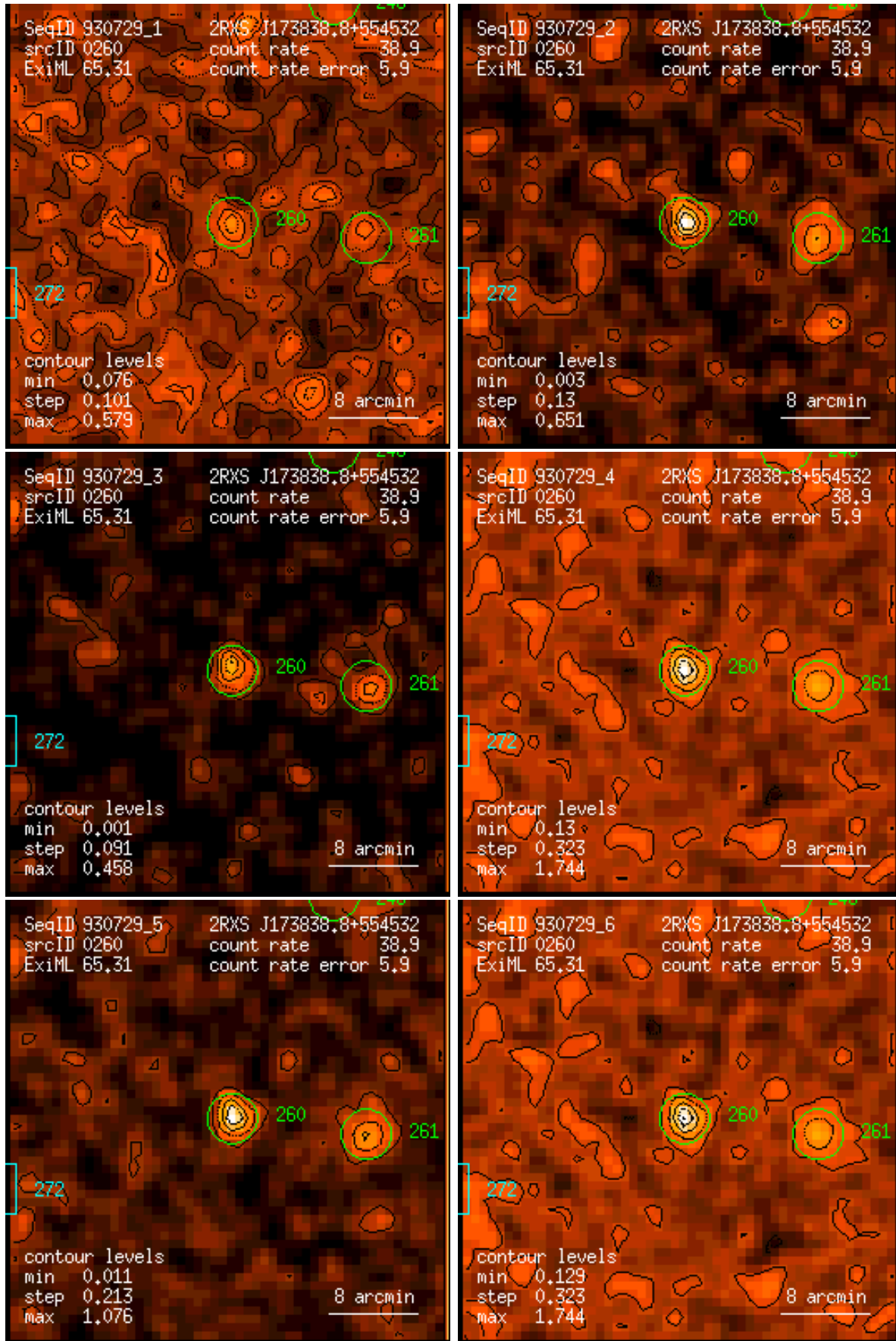
Figure 260: RASS 930729: detection 0260: band rate images, Gaussian filter: (1) PSPC channels 11 – 41, (2) 52 – 90, (3) 91 – 201, (4) 11 – 235, (5) 52 – 201, (6) 11 – 201. Broad band rates in counts/ks. Band rate contour levels in counts/ks/arcmin 2 .
