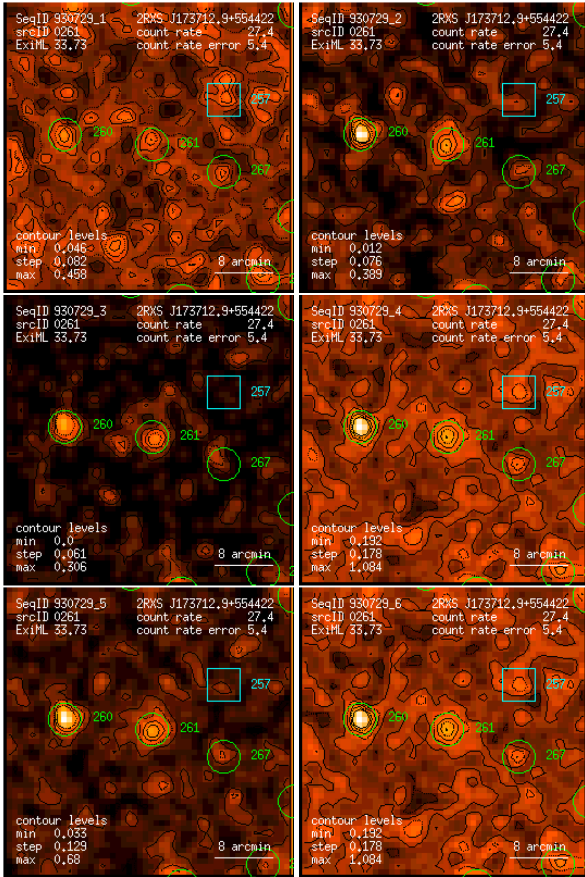
Figure 261: RASS 930729: detection 0261: band rate images, Gaussian filter: (1) PSPC channels 11 – 41, (2) 52 – 90, (3) 91 – 201, (4) 11 – 235, (5) 52 – 201, (6) 11 – 201. Broad band rates in counts/ks. Band rate contour levels in counts/ks/arcmin 2 .
