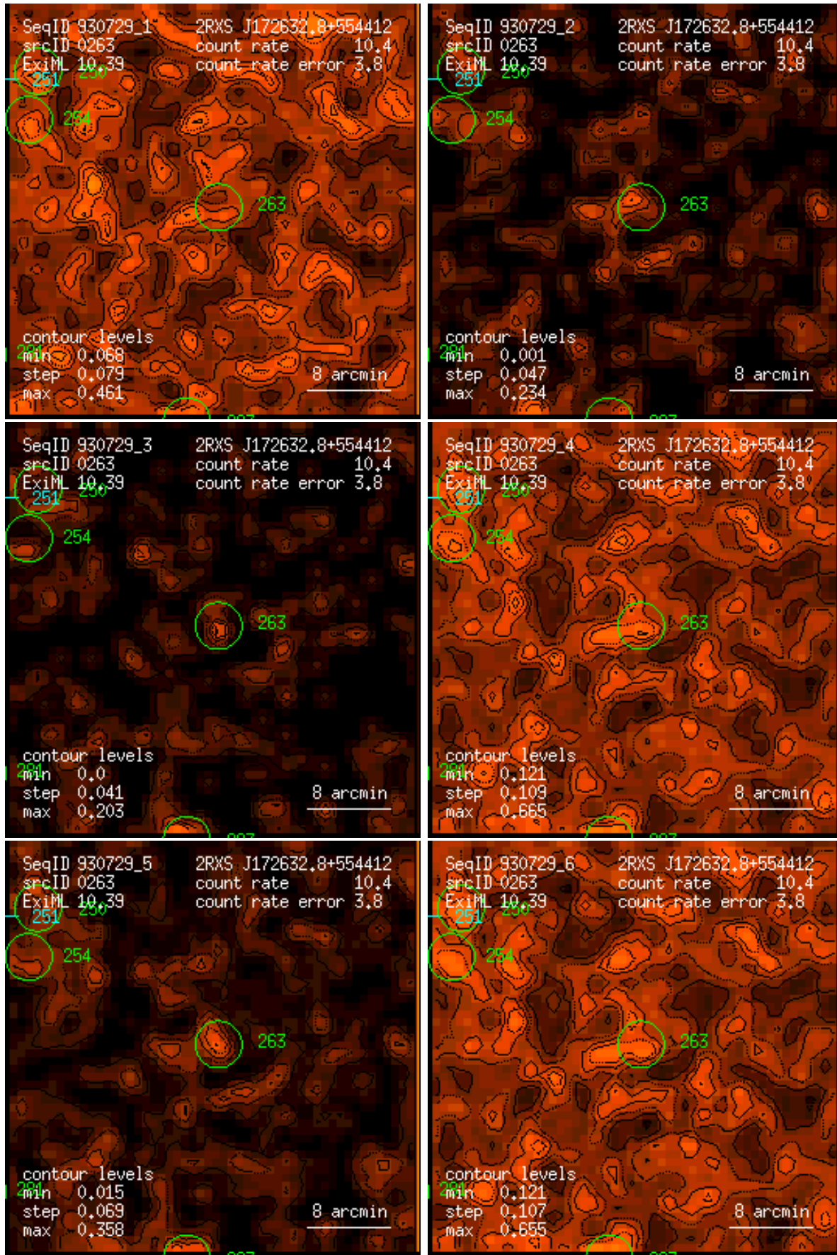
Figure 263: RASS 930729: detection 0263: band rate images, Gaussian filter: (1) PSPC channels 11 – 41, (2) 52 – 90, (3) 91 – 201, (4) 11 – 235, (5) 52 – 201, (6) 11 – 201. Broad band rates in counts/ks. Band rate contour levels in counts/ks/arcmin 2 .
