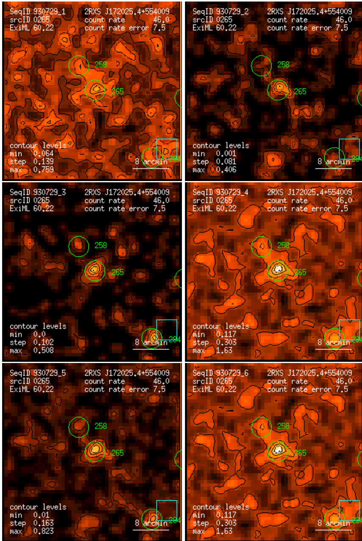
Figure 265: RASS 930729: detection 0265: band rate images, Gaussian filter: (1) PSPC channels 11 – 41, (2) 52 – 90, (3) 91 – 201, (4) 11 – 235, (5) 52 – 201, (6) 11 – 201. Broad band rates in counts/ks. Band rate contour levels in counts/ks/arcmin 2 .
