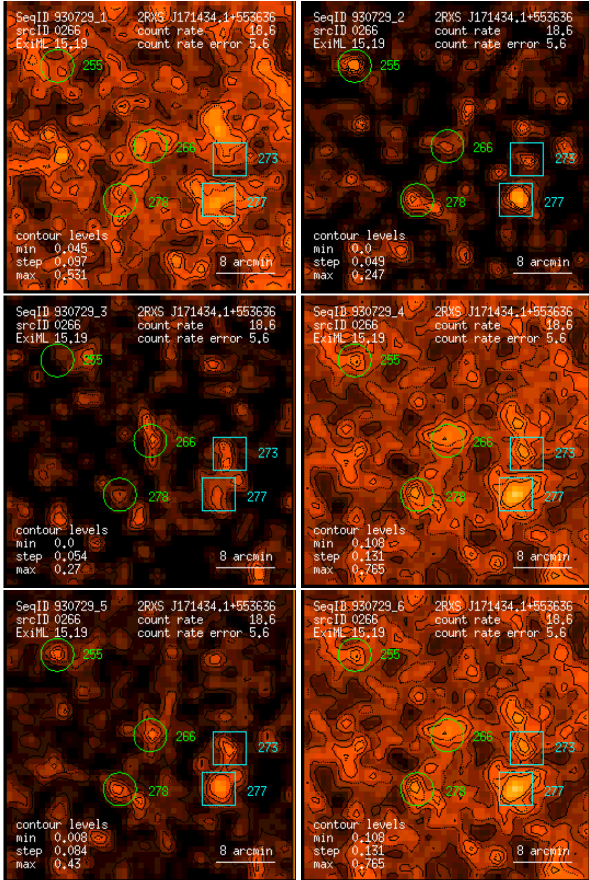
Figure 266: RASS 930729: detection 0266: band rate images, Gaussian filter: (1) PSPC channels 11 – 41, (2) 52 – 90, (3) 91 – 201, (4) 11 – 235, (5) 52 – 201, (6) 11 – 201. Broad band rates in counts/ks. Band rate contour levels in counts/ks/arcmin 2 .
