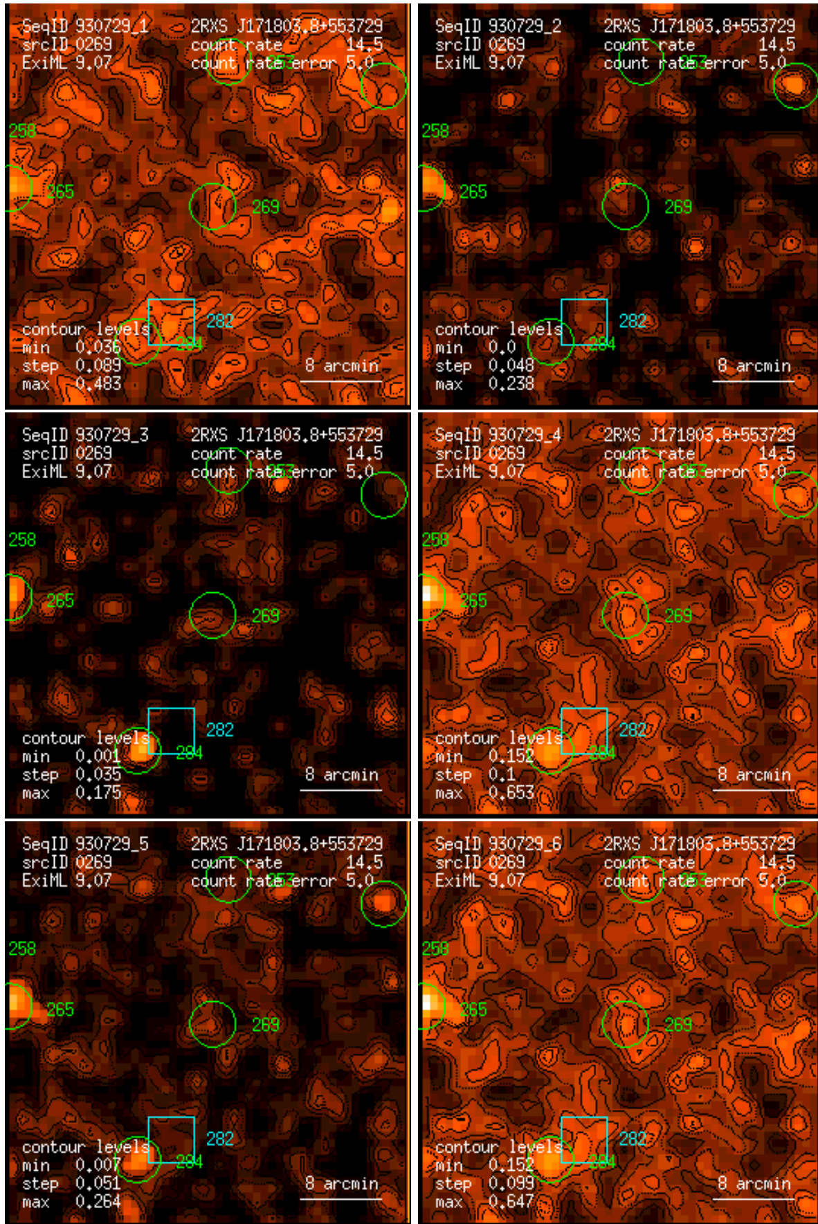
Figure 269: RASS 930729: detection 0269: band rate images, Gaussian filter: (1) PSPC channels 11 – 41, (2) 52 – 90, (3) 91 – 201, (4) 11 – 235, (5) 52 – 201, (6) 11 – 201. Broad band rates in counts/ks. Band rate contour levels in counts/ks/arcmin 2 .
