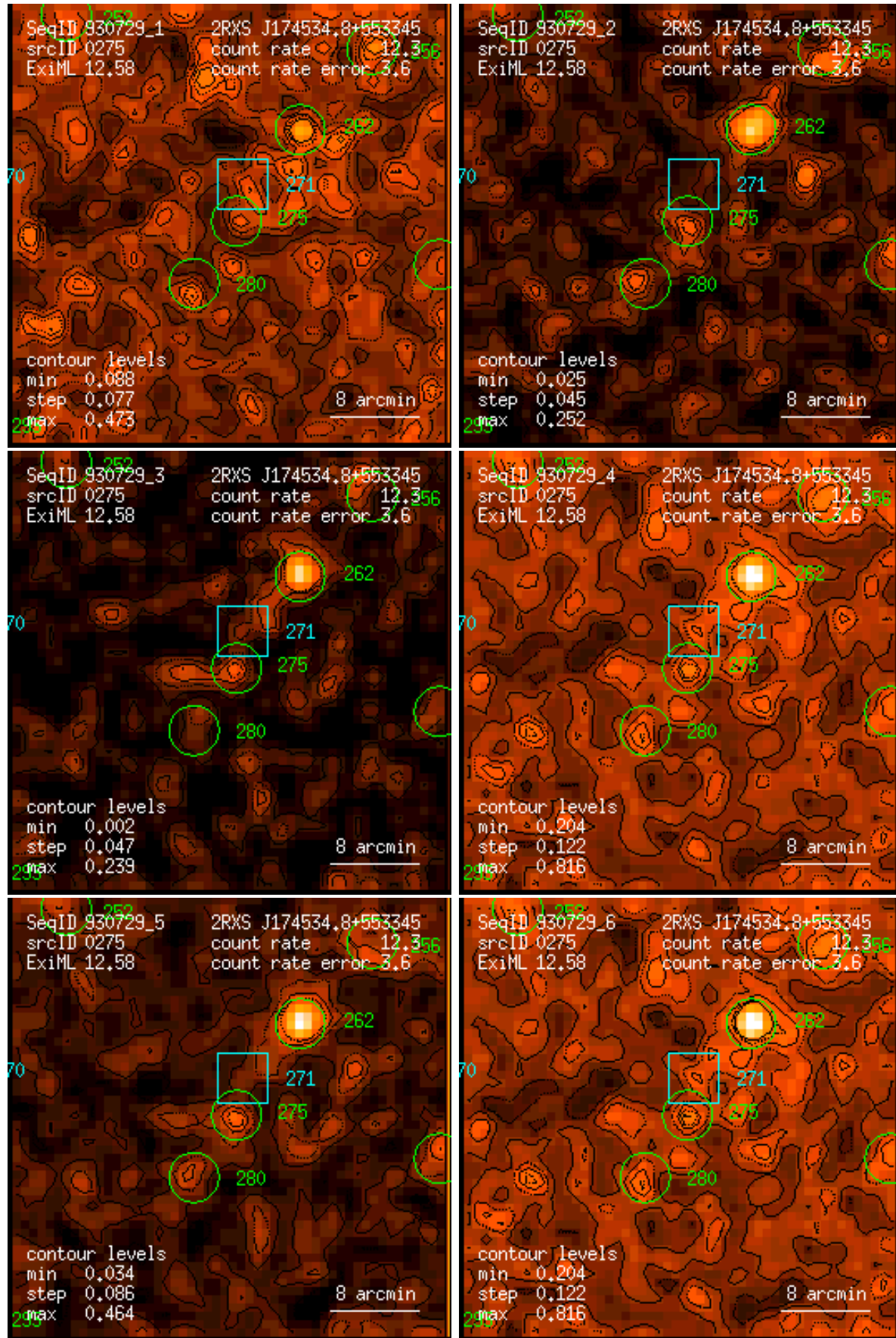
Figure 275: RASS 930729: detection 0275: band rate images, Gaussian filter: (1) PSPC channels 11 – 41, (2) 52 – 90, (3) 91 – 201, (4) 11 – 235, (5) 52 – 201, (6) 11 – 201. Broad band rates in counts/ks. Band rate contour levels in counts/ks/arcmin 2 .
