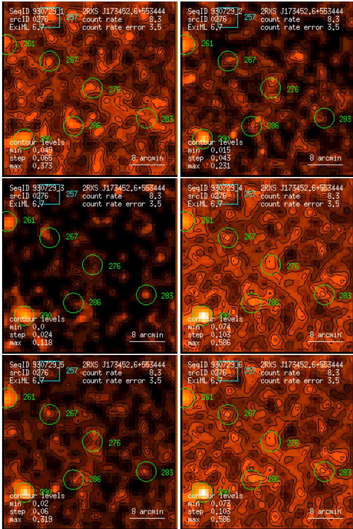
Figure 276: RASS 930729: detection 0276: band rate images, Gaussian filter: (1) PSPC channels 11 – 41, (2) 52 – 90, (3) 91 – 201, (4) 11 – 235, (5) 52 – 201, (6) 11 – 201. Broad band rates in counts/ks. Band rate contour levels in counts/ks/arcmin 2 .
