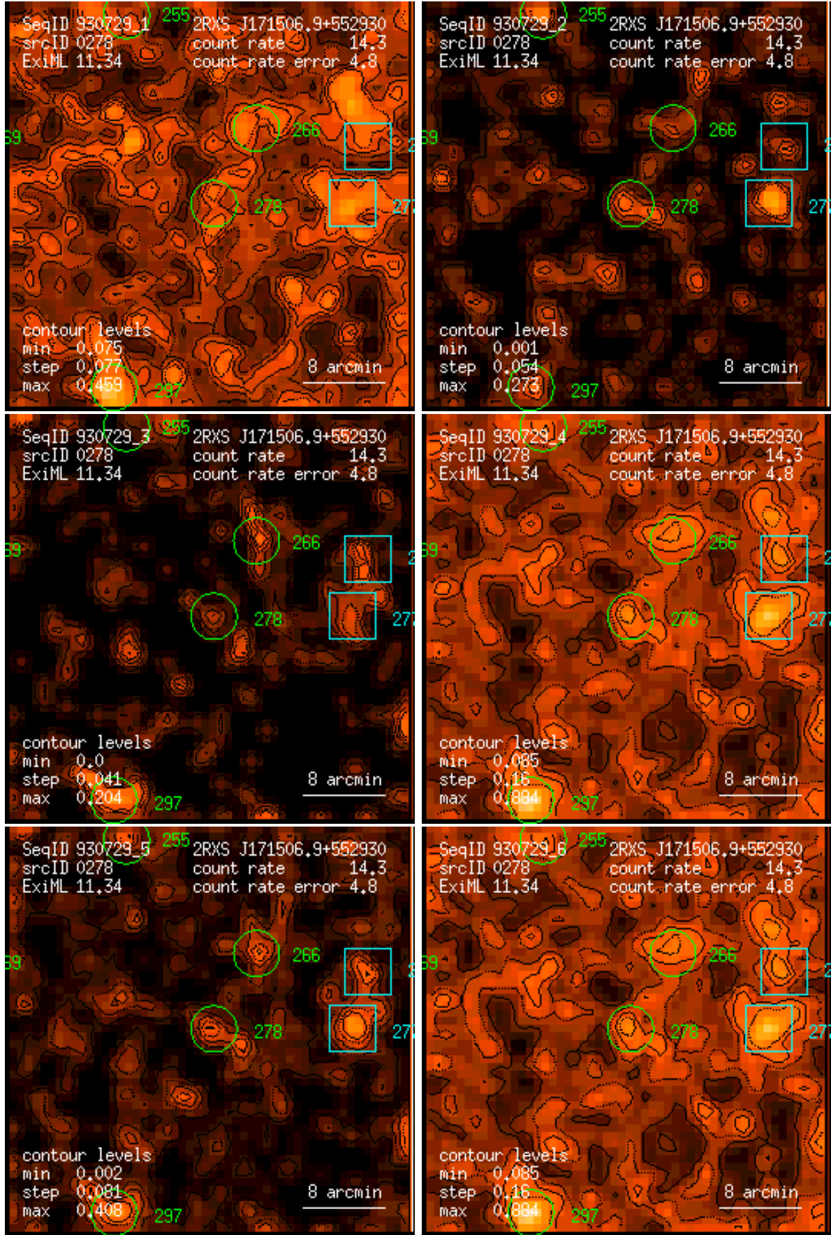
Figure 278: RASS 930729: detection 0278: band rate images, Gaussian filter: (1) PSPC channels 11 – 41, (2) 52 – 90, (3) 91 – 201, (4) 11 – 235, (5) 52 – 201, (6) 11 – 201. Broad band rates in counts/ks. Band rate contour levels in counts/ks/arcmin 2 .
