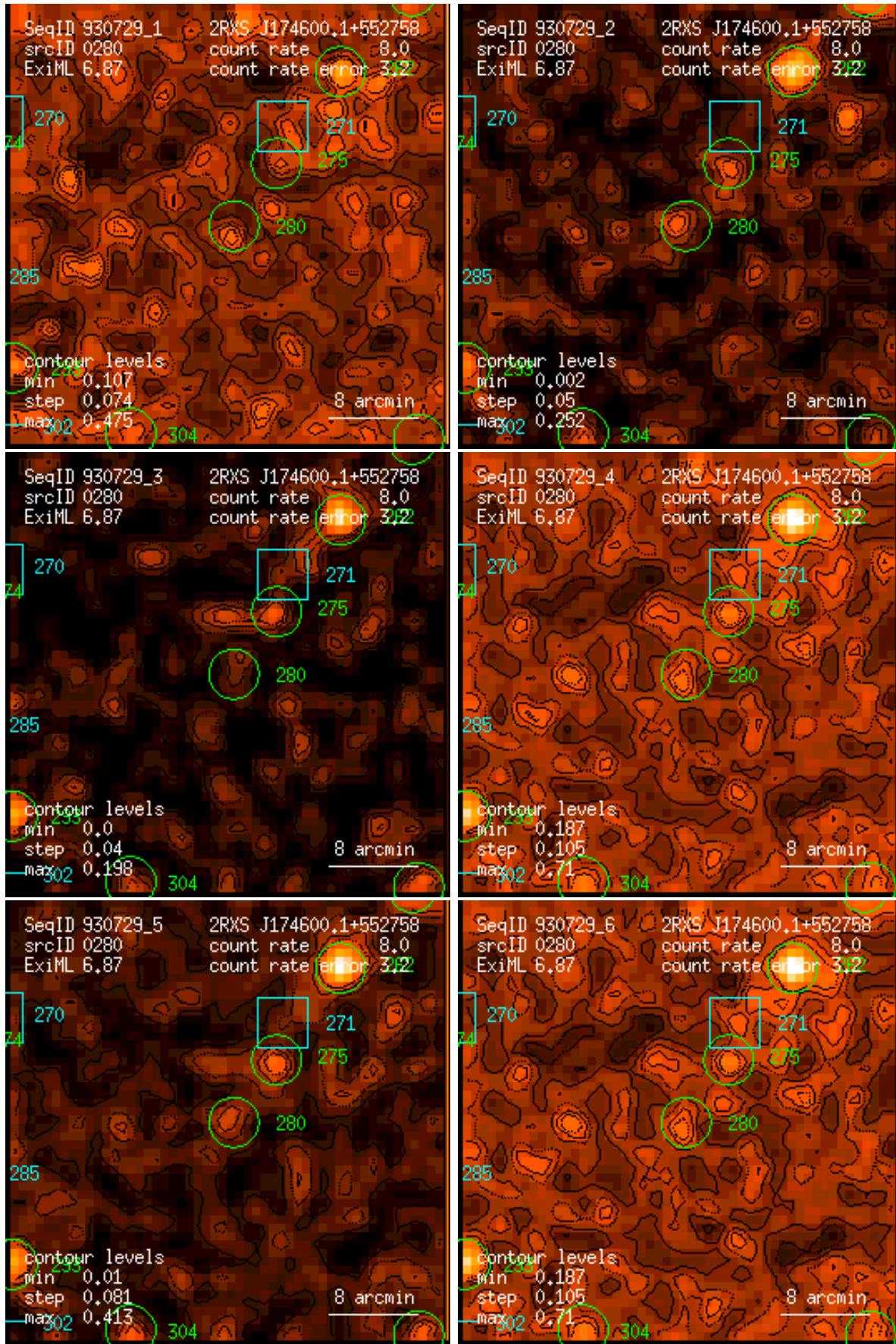
Figure 280: RASS 930729: detection 0280: band rate images, Gaussian filter: (1) PSPC channels 11 – 41, (2) 52 – 90, (3) 91 – 201, (4) 11 – 235, (5) 52 – 201, (6) 11 – 201. Broad band rates in counts/ks. Band rate contour levels in counts/ks/arcmin 2 .
