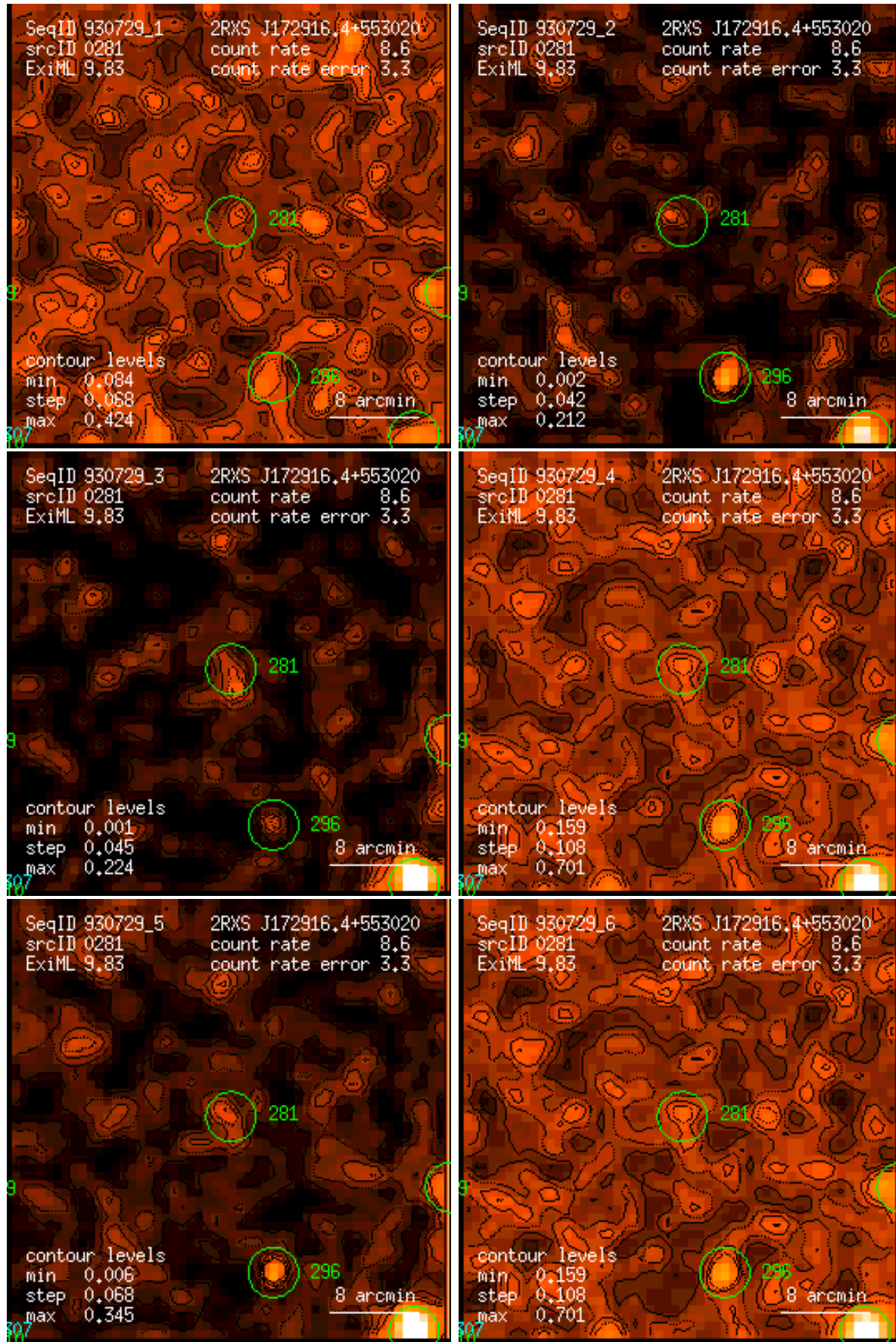
Figure 281: RASS 930729: detection 0281: band rate images, Gaussian filter: (1) PSPC channels 11 – 41, (2) 52 – 90, (3) 91 – 201, (4) 11 – 235, (5) 52 – 201, (6) 11 – 201. Broad band rates in counts/ks. Band rate contour levels in counts/ks/arcmin 2 .
