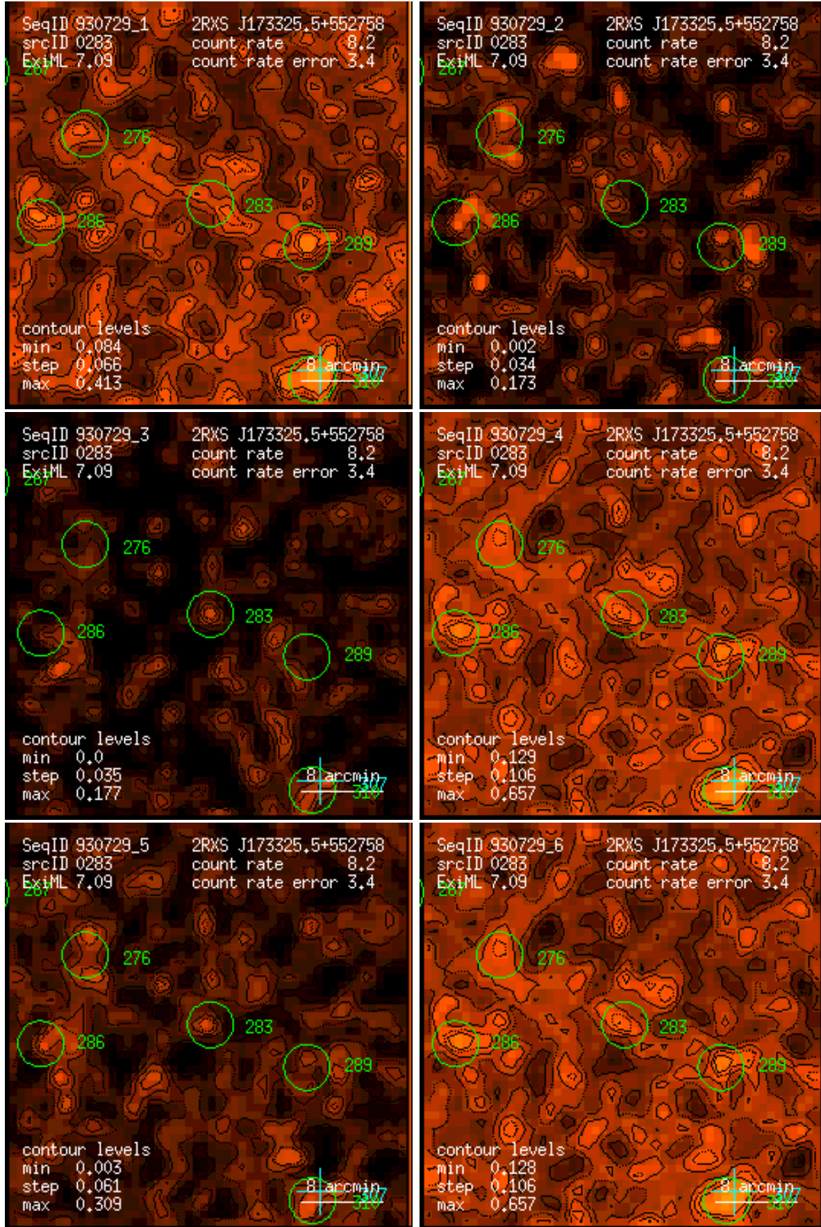
Figure 283: RASS 930729: detection 0283: band rate images, Gaussian filter: (1) PSPC channels 11 – 41, (2) 52 – 90, (3) 91 – 201, (4) 11 – 235, (5) 52 – 201, (6) 11 – 201. Broad band rates in counts/ks. Band rate contour levels in counts/ks/arcmin 2 .
