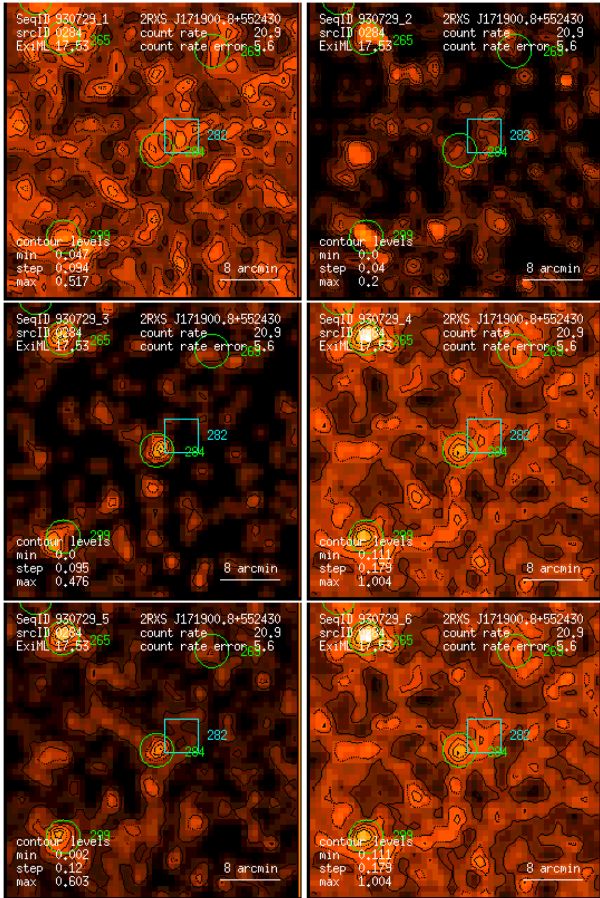
Figure 284: RASS 930729: detection 0284: band rate images, Gaussian filter: (1) PSPC channels 11 – 41, (2) 52 – 90, (3) 91 – 201, (4) 11 – 235, (5) 52 – 201, (6) 11 – 201. Broad band rates in counts/ks. Band rate contour levels in counts/ks/arcmin 2 .
