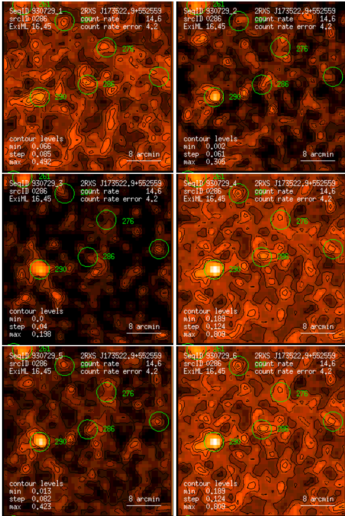
Figure 286: RASS 930729: detection 0286: band rate images, Gaussian filter: (1) PSPC channels 11 – 41, (2) 52 – 90, (3) 91 – 201, (4) 11 – 235, (5) 52 – 201, (6) 11 – 201. Broad band rates in counts/ks. Band rate contour levels in counts/ks/arcmin 2 .
