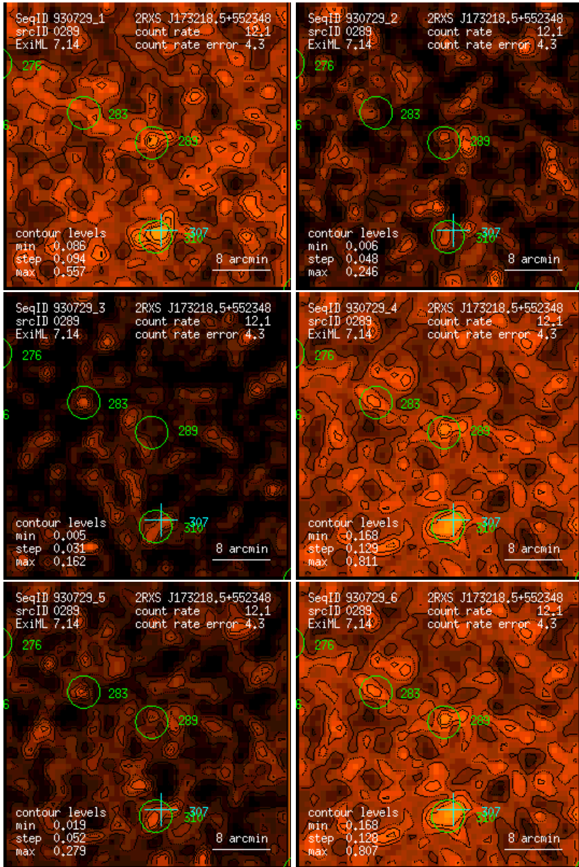
Figure 289: RASS 930729: detection 0289: band rate images, Gaussian filter: (1) PSPC channels 11 – 41, (2) 52 – 90, (3) 91 – 201, (4) 11 – 235, (5) 52 – 201, (6) 11 – 201. Broad band rates in counts/ks. Band rate contour levels in counts/ks/arcmin 2 .
