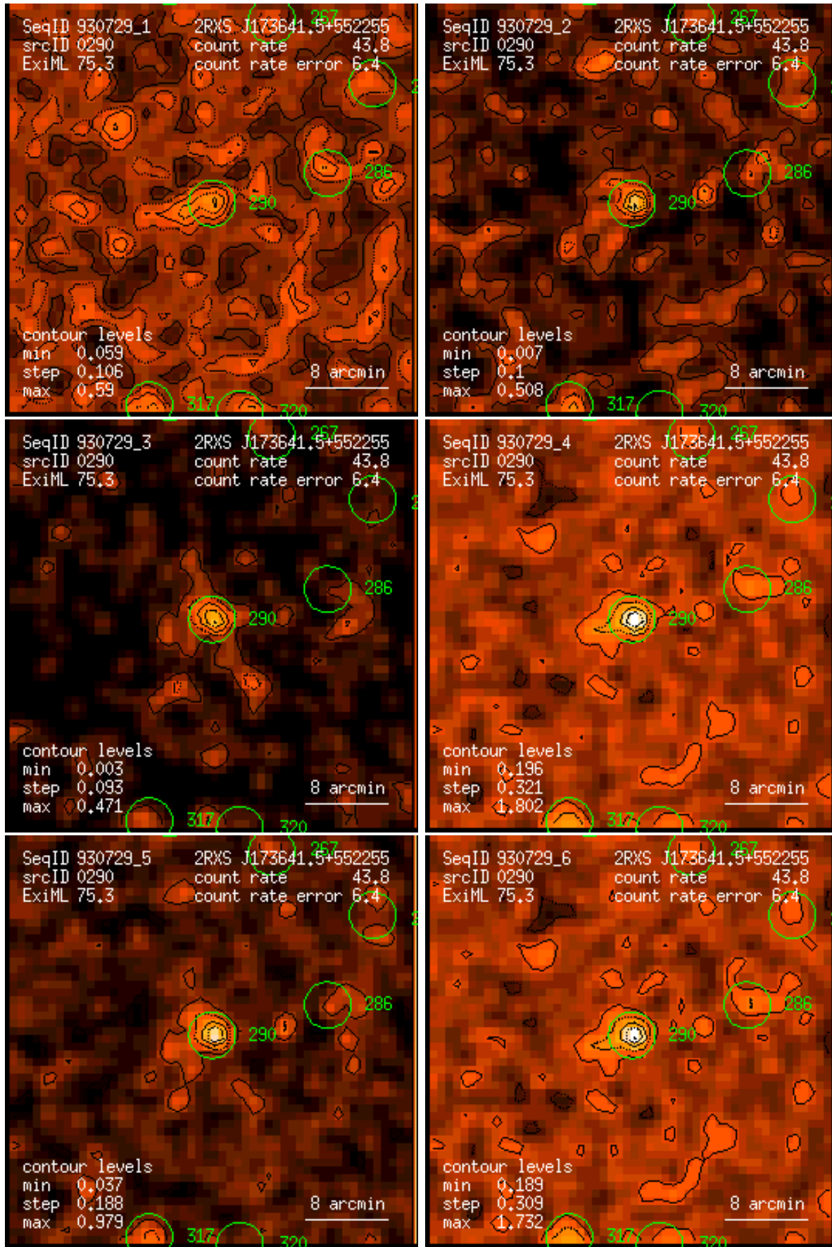
Figure 290: RASS 930729: detection 0290: band rate images, Gaussian filter: (1) PSPC channels 11 – 41, (2) 52 – 90, (3) 91 – 201, (4) 11 – 235, (5) 52 – 201, (6) 11 – 201. Broad band rates in counts/ks. Band rate contour levels in counts/ks/arcmin 2 .
