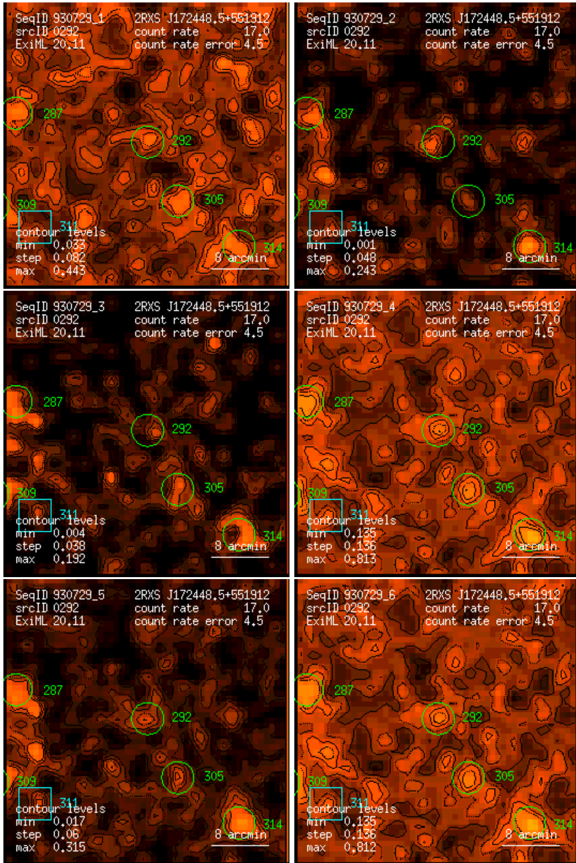
Figure 292: RASS 930729: detection 0292: band rate images, Gaussian filter: (1) PSPC channels 11 – 41, (2) 52 – 90, (3) 91 – 201, (4) 11 – 235, (5) 52 – 201, (6) 11 – 201. Broad band rates in counts/ks. Band rate contour levels in counts/ks/arcmin 2 .
