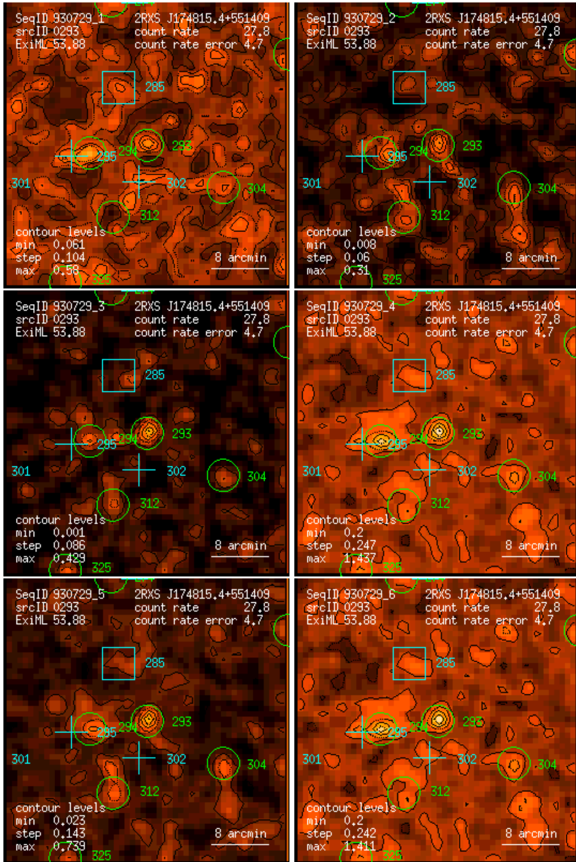
Figure 293: RASS 930729: detection 0293: band rate images, Gaussian filter: (1) PSPC channels 11 – 41, (2) 52 – 90, (3) 91 – 201, (4) 11 – 235, (5) 52 – 201, (6) 11 – 201. Broad band rates in counts/ks. Band rate contour levels in counts/ks/arcmin 2 .
