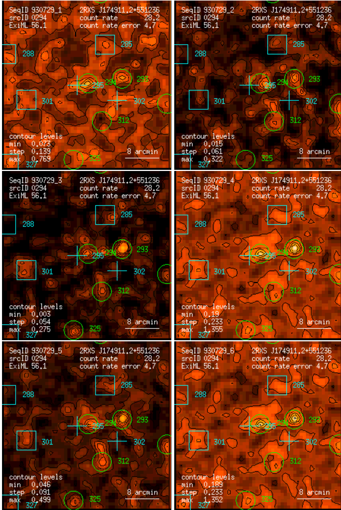
Figure 294: RASS 930729: detection 0294: band rate images, Gaussian filter: (1) PSPC channels 11 – 41, (2) 52 – 90, (3) 91 – 201, (4) 11 – 235, (5) 52 – 201, (6) 11 – 201. Broad band rates in counts/ks. Band rate contour levels in counts/ks/arcmin 2 .
