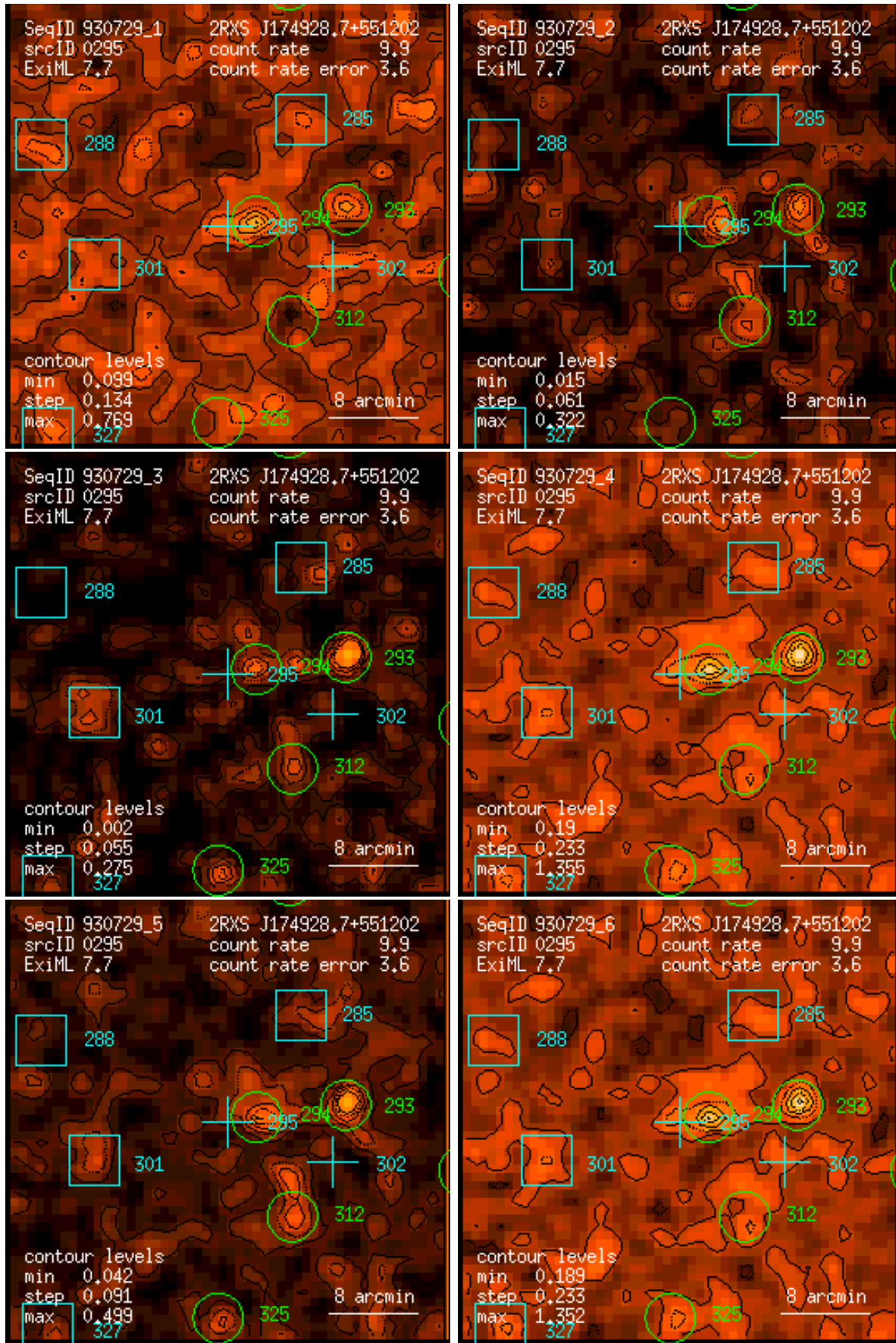
Figure 295: RASS 930729: detection 0295: band rate images, Gaussian filter: (1) PSPC channels 11 – 41, (2) 52 – 90, (3) 91 – 201, (4) 11 – 235, (5) 52 – 201, (6) 11 – 201. Broad band rates in counts/ks. Band rate contour levels in counts/ks/arcmin 2 .
