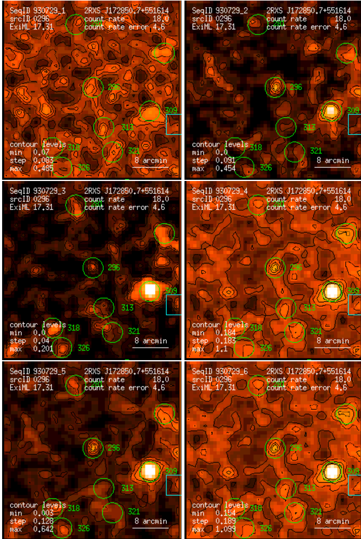
Figure 296: RASS 930729: detection 0296: band rate images, Gaussian filter: (1) PSPC channels 11 – 41, (2) 52 – 90, (3) 91 – 201, (4) 11 – 235, (5) 52 – 201, (6) 11 – 201. Broad band rates in counts/ks. Band rate contour levels in counts/ks/arcmin 2 .
