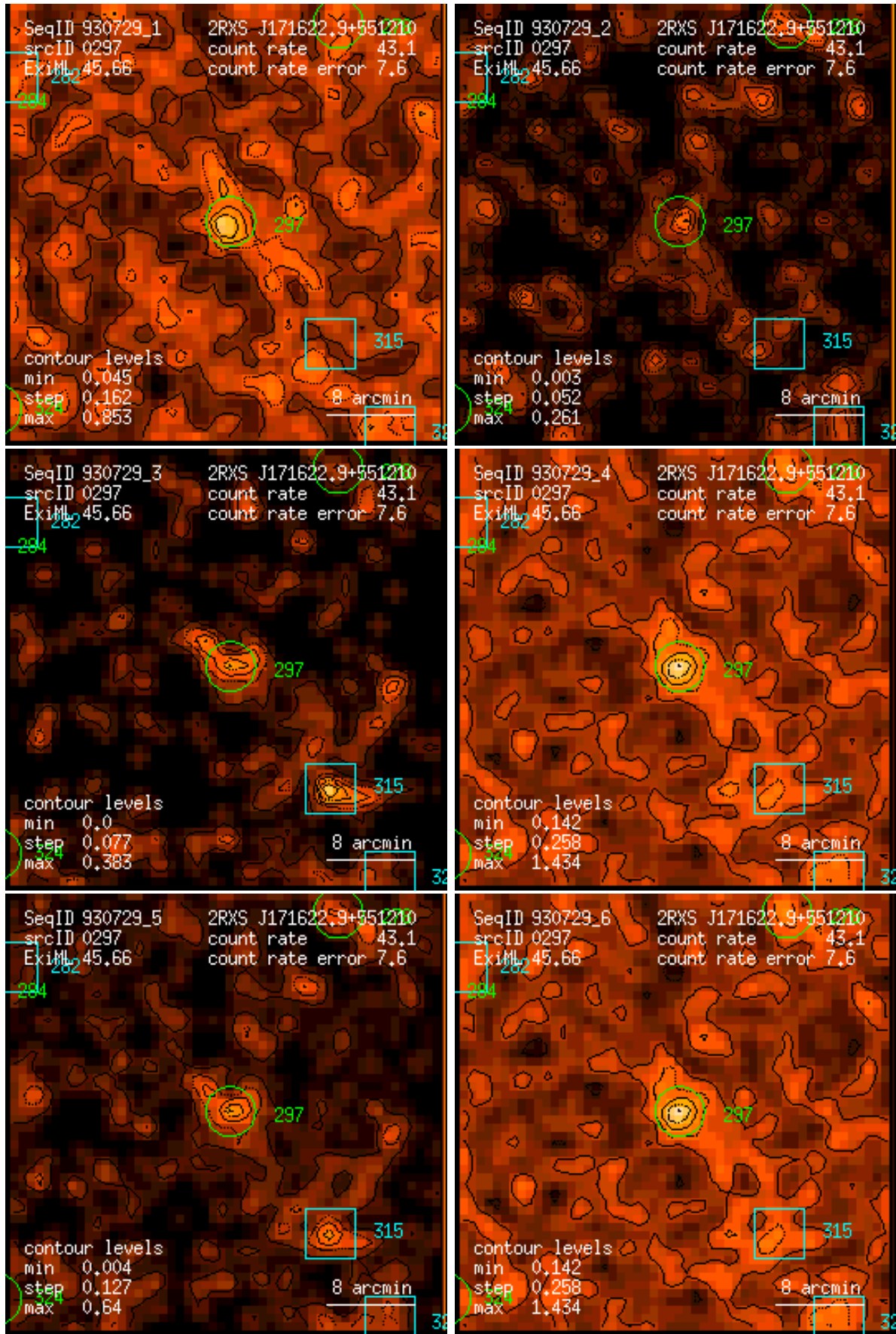
Figure 297: RASS 930729: detection 0297: band rate images, Gaussian filter: (1) PSPC channels 11 – 41, (2) 52 – 90, (3) 91 – 201, (4) 11 – 235, (5) 52 – 201, (6) 11 – 201. Broad band rates in counts/ks. Band rate contour levels in counts/ks/arcmin 2 .
