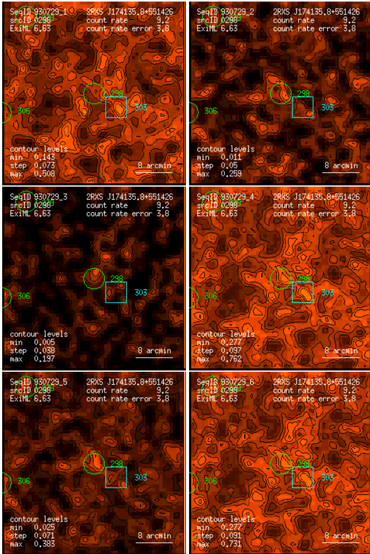
Figure 298: RASS 930729: detection 0298: band rate images, Gaussian filter: (1) PSPC channels 11 – 41, (2) 52 – 90, (3) 91 – 201, (4) 11 – 235, (5) 52 – 201, (6) 11 – 201. Broad band rates in counts/ks. Band rate contour levels in counts/ks/arcmin 2 .
