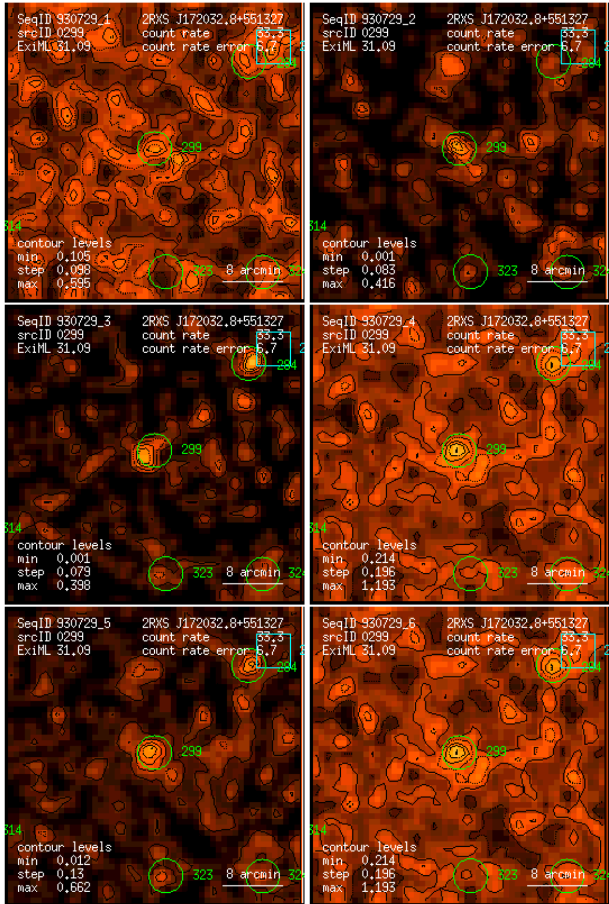
Figure 299: RASS 930729: detection 0299: band rate images, Gaussian filter: (1) PSPC channels 11 – 41, (2) 52 – 90, (3) 91 – 201, (4) 11 – 235, (5) 52 – 201, (6) 11 – 201. Broad band rates in counts/ks. Band rate contour levels in counts/ks/arcmin 2 .
