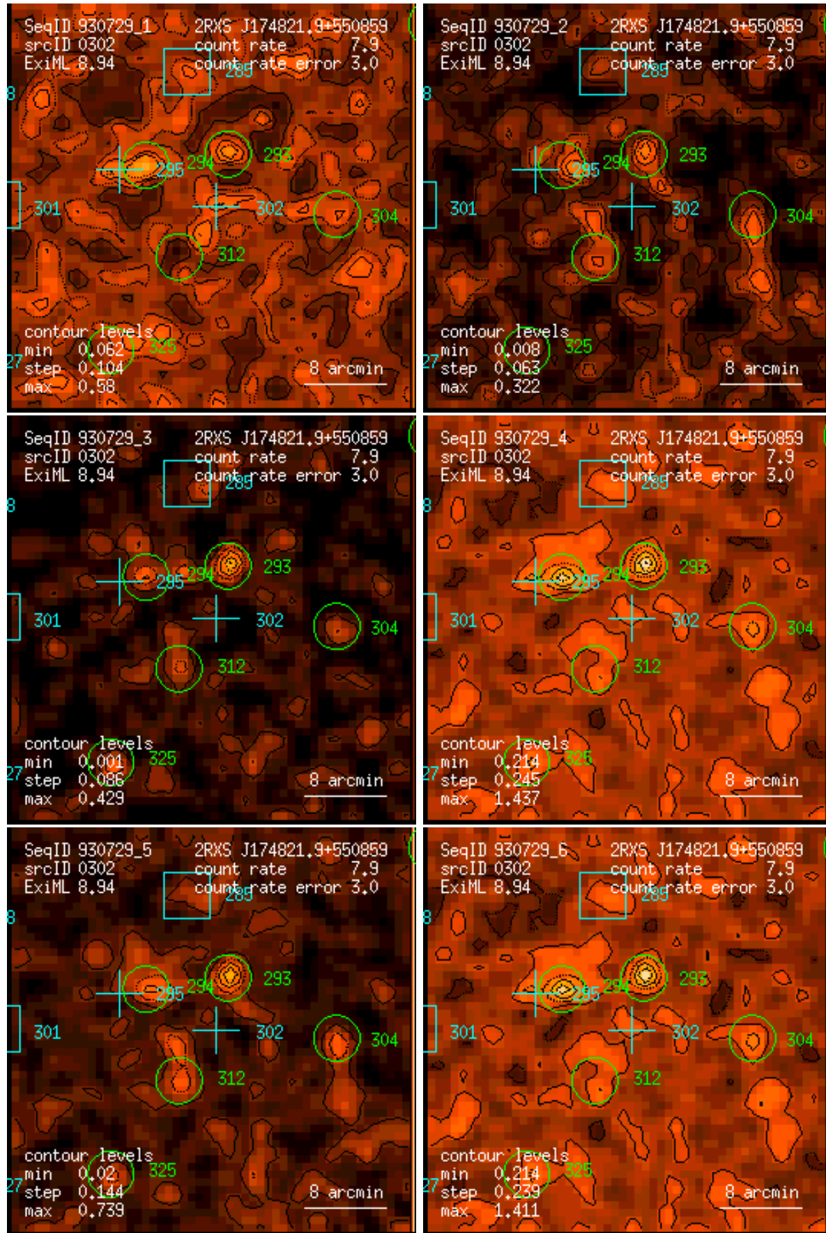
Figure 302: RASS 930729: detection 0302: band rate images, Gaussian filter: (1) PSPC channels 11 – 41, (2) 52 – 90, (3) 91 – 201, (4) 11 – 235, (5) 52 – 201, (6) 11 – 201. Broad band rates in counts/ks. Band rate contour levels in counts/ks/arcmin 2 .
