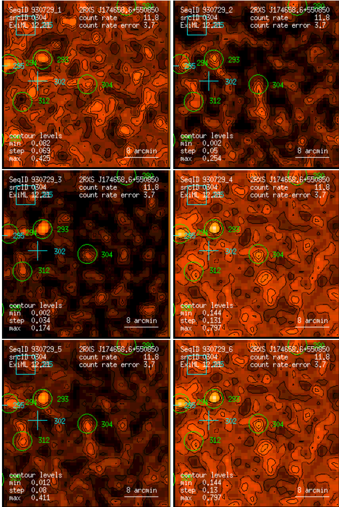
Figure 304: RASS 930729: detection 0304: band rate images, Gaussian filter: (1) PSPC channels 11 – 41, (2) 52 – 90, (3) 91 – 201, (4) 11 – 235, (5) 52 – 201, (6) 11 – 201. Broad band rates in counts/ks. Band rate contour levels in counts/ks/arcmin 2 .
