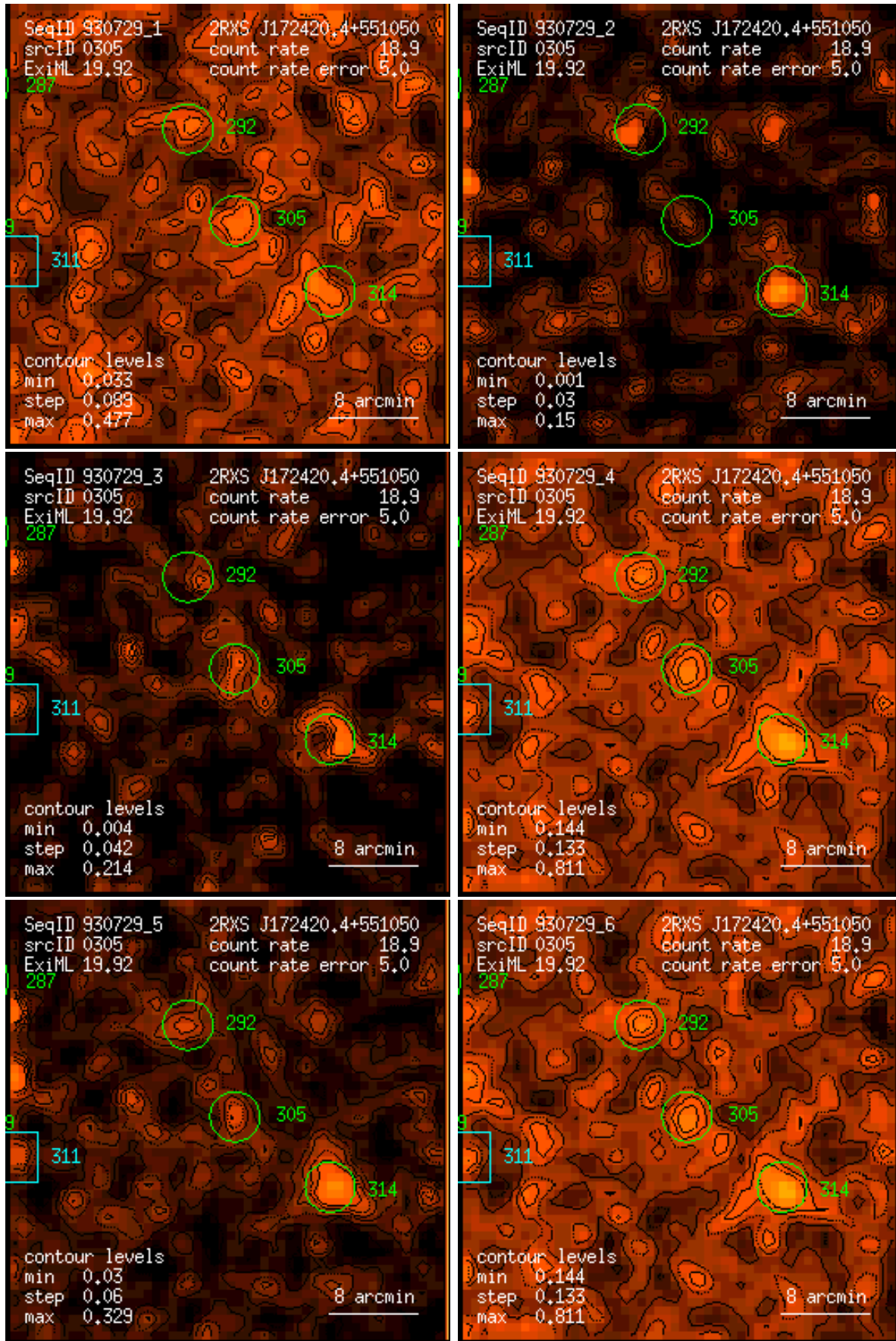
Figure 305: RASS 930729: detection 0305: band rate images, Gaussian filter: (1) PSPC channels 11 – 41, (2) 52 – 90, (3) 91 – 201, (4) 11 – 235, (5) 52 – 201, (6) 11 – 201. Broad band rates in counts/ks. Band rate contour levels in counts/ks/arcmin 2 .
