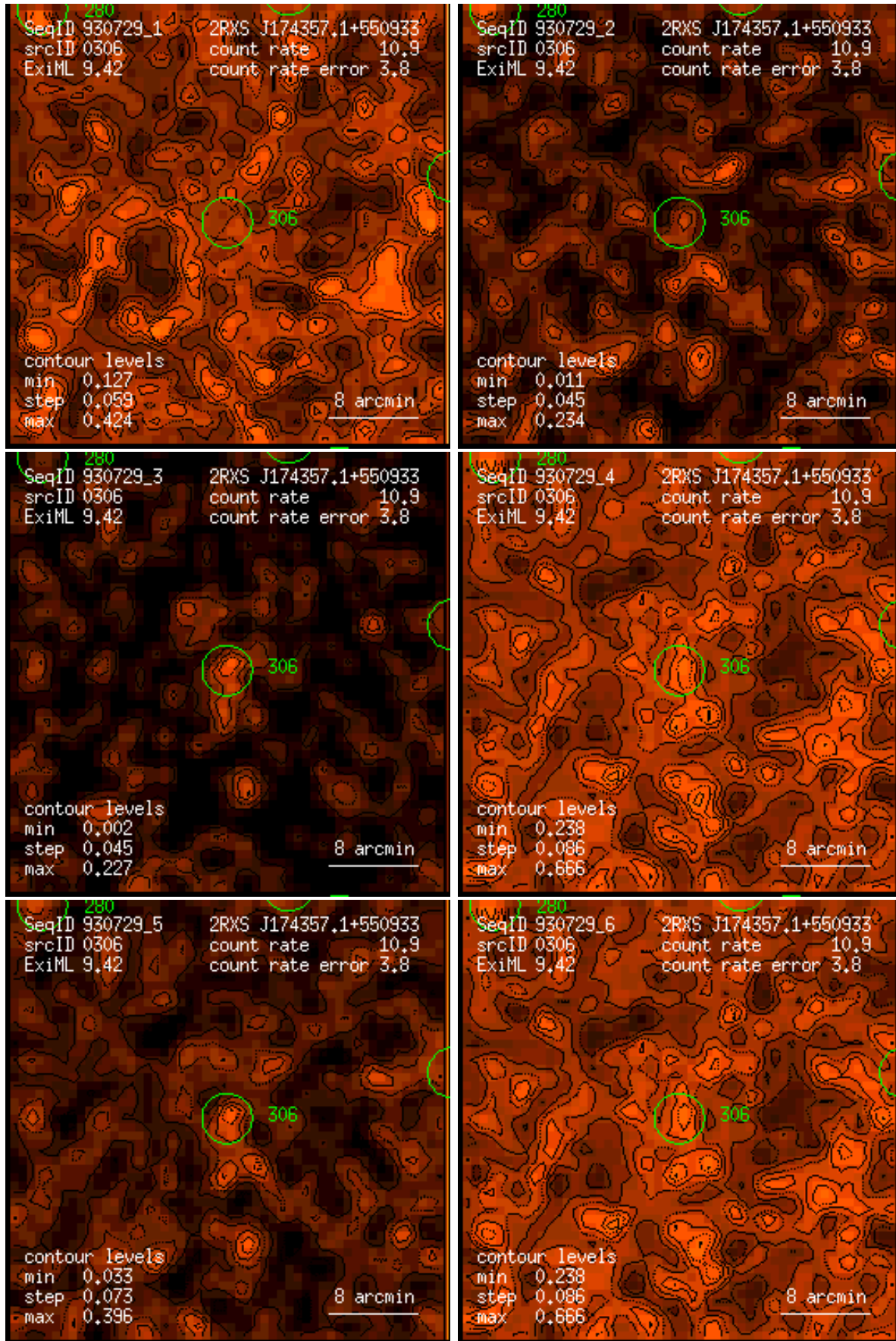
Figure 306: RASS 930729: detection 0306: band rate images, Gaussian filter: (1) PSPC channels 11 – 41, (2) 52 – 90, (3) 91 – 201, (4) 11 – 235, (5) 52 – 201, (6) 11 – 201. Broad band rates in counts/ks. Band rate contour levels in counts/ks/arcmin 2 .
