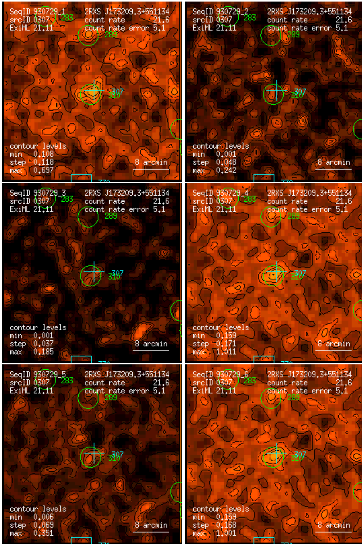
Figure 307: RASS 930729: detection 0307: band rate images, Gaussian filter: (1) PSPC channels 11 – 41, (2) 52 – 90, (3) 91 – 201, (4) 11 – 235, (5) 52 – 201, (6) 11 – 201. Broad band rates in counts/ks. Band rate contour levels in counts/ks/arcmin 2 .
