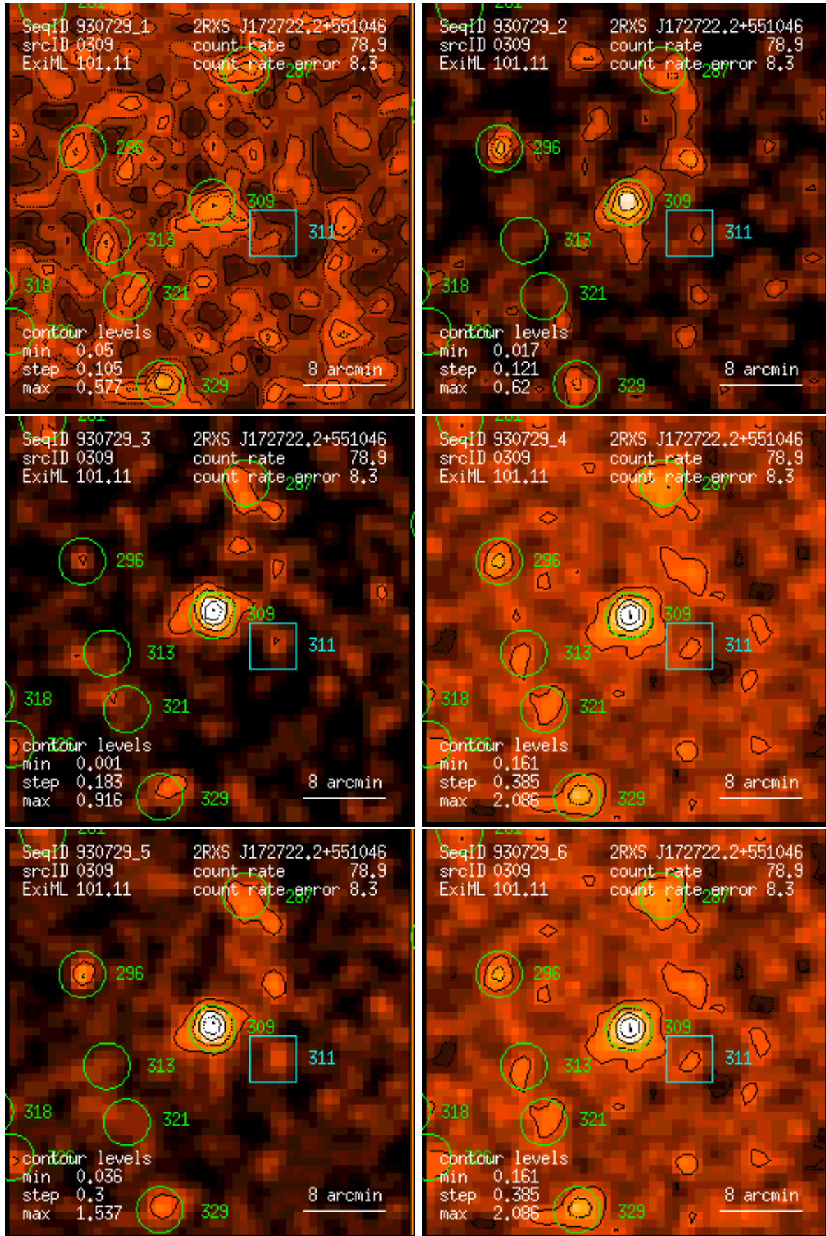
Figure 309: RASS 930729: detection 0309: band rate images, Gaussian filter: (1) PSPC channels 11 – 41, (2) 52 – 90, (3) 91 – 201, (4) 11 – 235, (5) 52 – 201, (6) 11 – 201. Broad band rates in counts/ks. Band rate contour levels in counts/ks/arcmin 2 .
